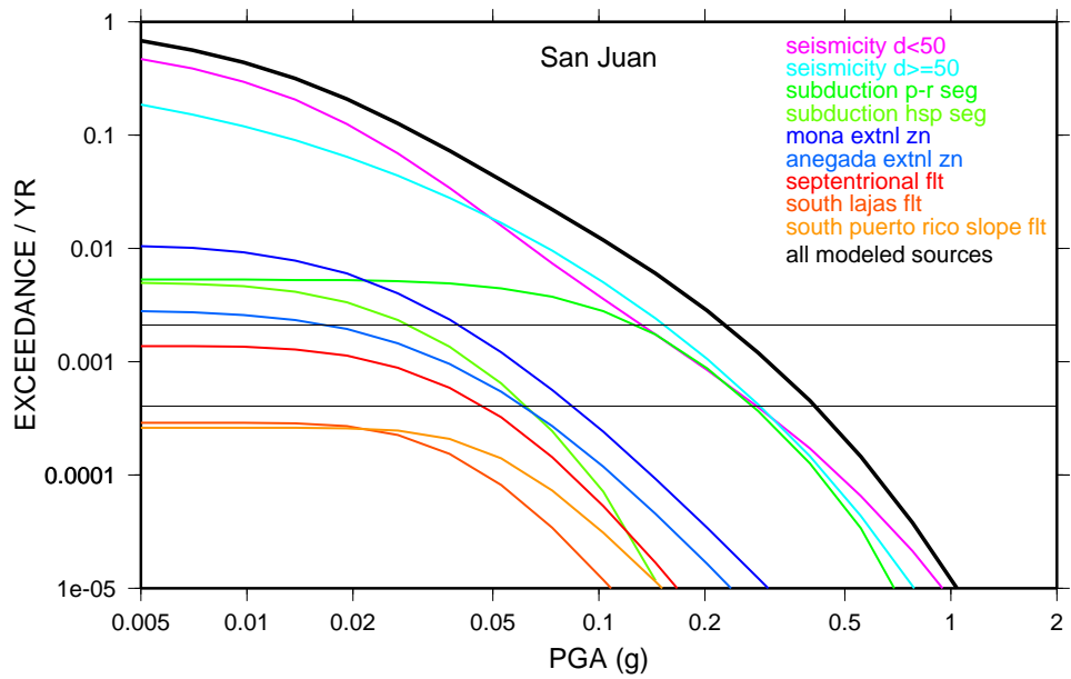
Fig.13a: PGA hazard curves for San Juan.
