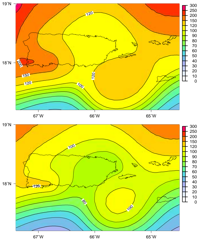
Fig.11: 0.2-second spectral acceleration (%g) with 2% probability of exceedance in 50 years from all modeled sources. Compare 50% (top) and 10% (bottom) weights for Motazedian & Atkinson (2003) attenuation.
