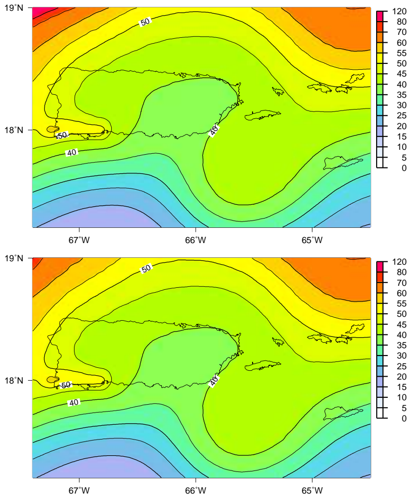
Fig.10: PGA (%g) with 2% probability of exceedance in 50 years from all modeled sources. Compare 9-mm/yr (top) and 1-mm/yr (bottom) scenarios for South Puerto Rico Slope fault zone (440-year and 3900-year recurrence, respectively).
