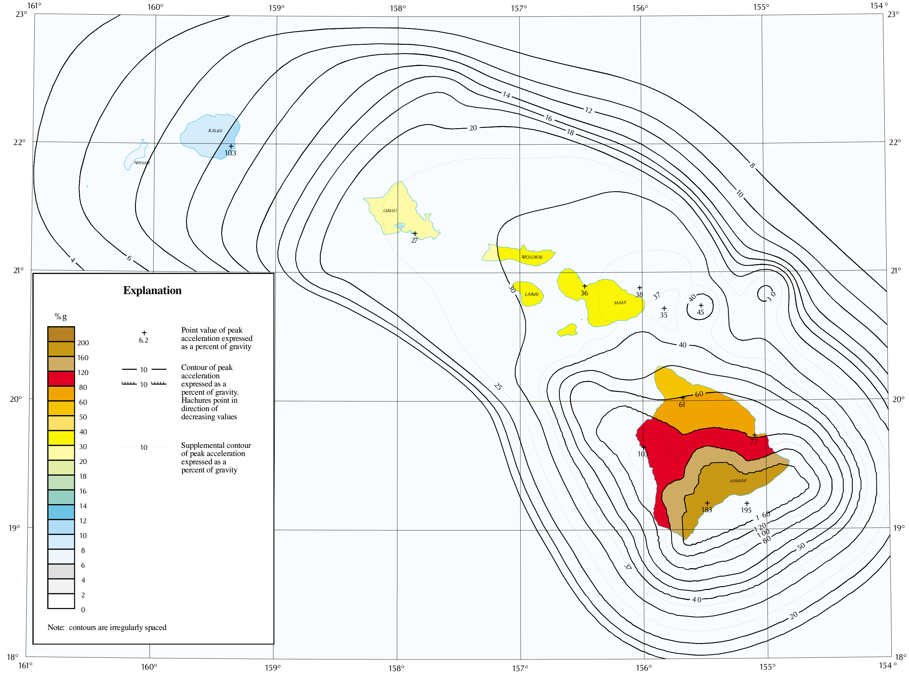
PEAK HORIZONTAL ACCELERATION WITH 2% PROBABILITY OF EXCEEDANCE IN 50 YEARS
