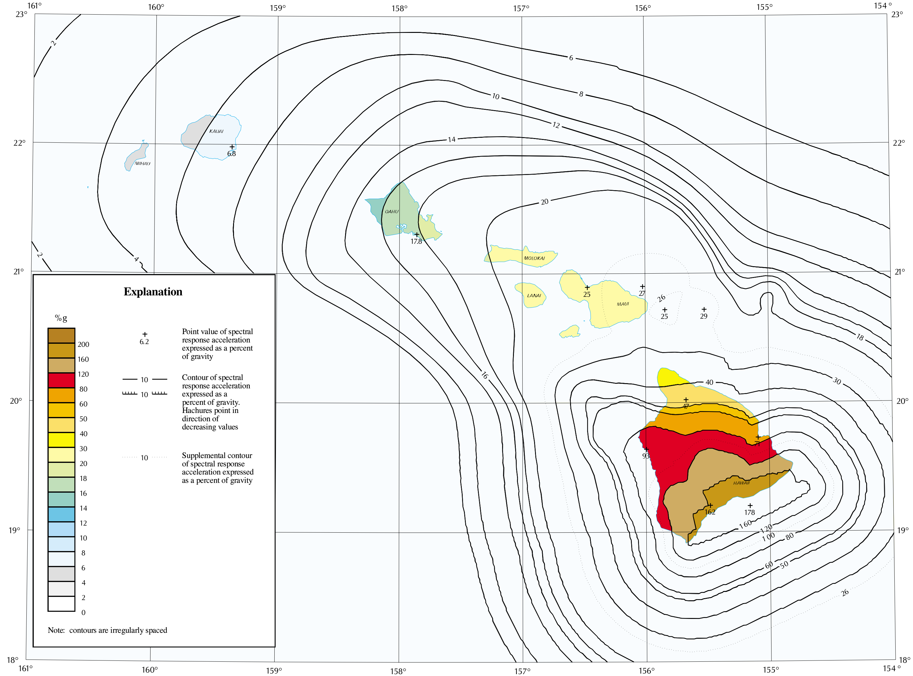
HORIZONTAL SPECTRAL RESPONSE ACCELERATION FOR 1.0 SECOND PERIOD (5% OF CRITICAL DAMPING) WITH 2% PROBABILITY OF EXCEEDANCE IN 50 YEARS
