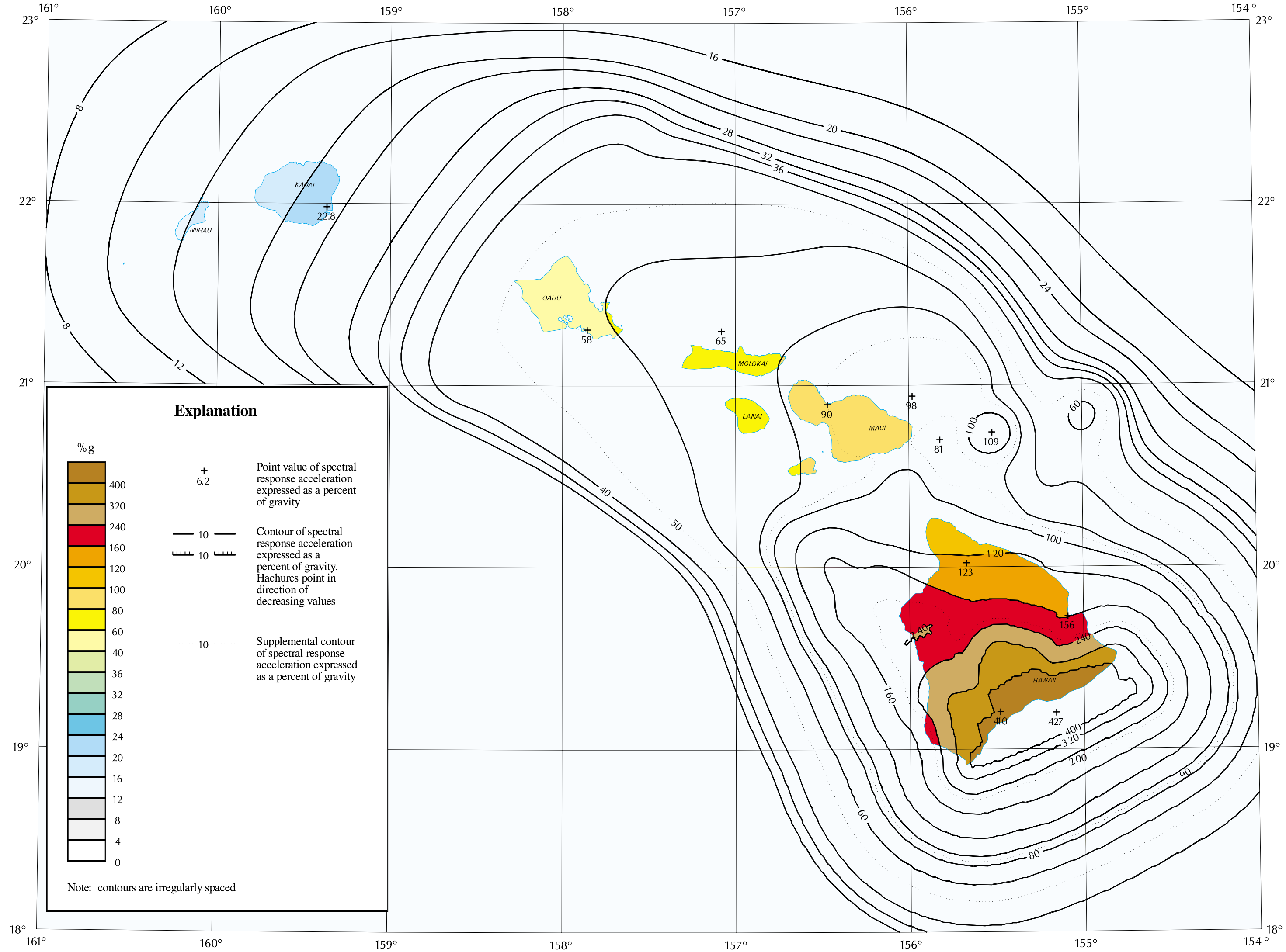
HORIZONTAL SPECTRAL RESPONSE ACCELERATION FOR 0.3 SECOND PERIOD (5% OF CRITICAL DAMPING) WITH 2% PROBABILITY OF EXCEEDANCE IN 50 YEARS
