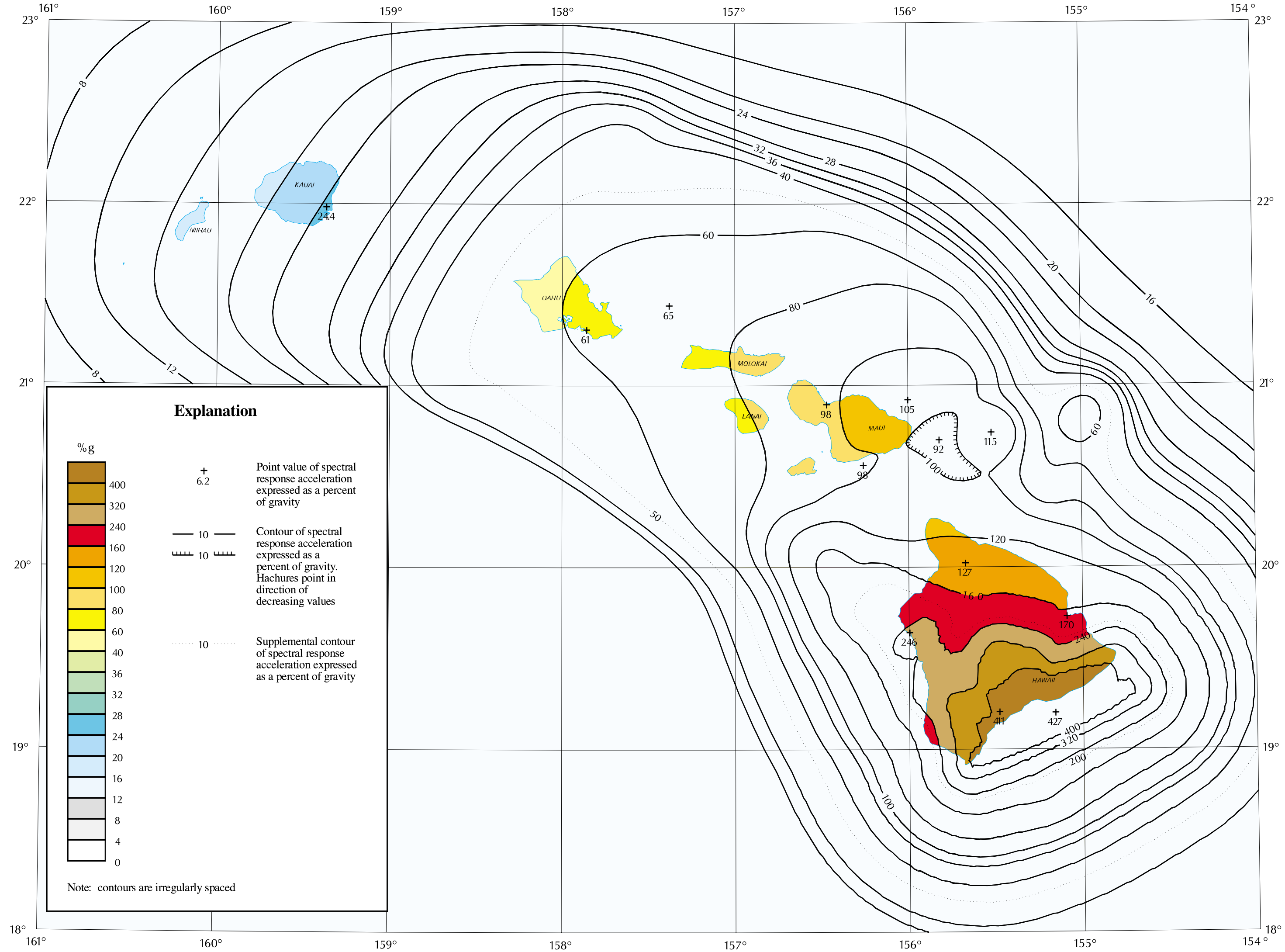
HORIZONTAL SPECTRAL RESPONSE ACCELERATION FOR 0.2 SECOND PERIOD (5% OF CRITICAL DAMPING) WITH 2% PROBABILITY OF EXCEEDANCE IN 50 YEARS
