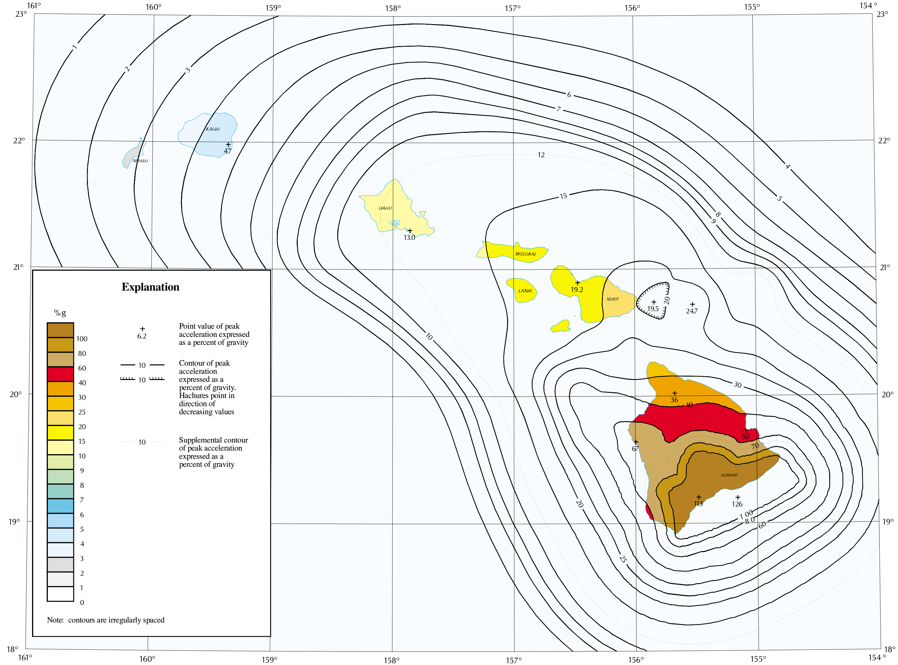
PEAK HORIZONTAL ACCELERATION WITH 10% PROBABILITY OF EXCEEDANCE IN 50 YEARS
