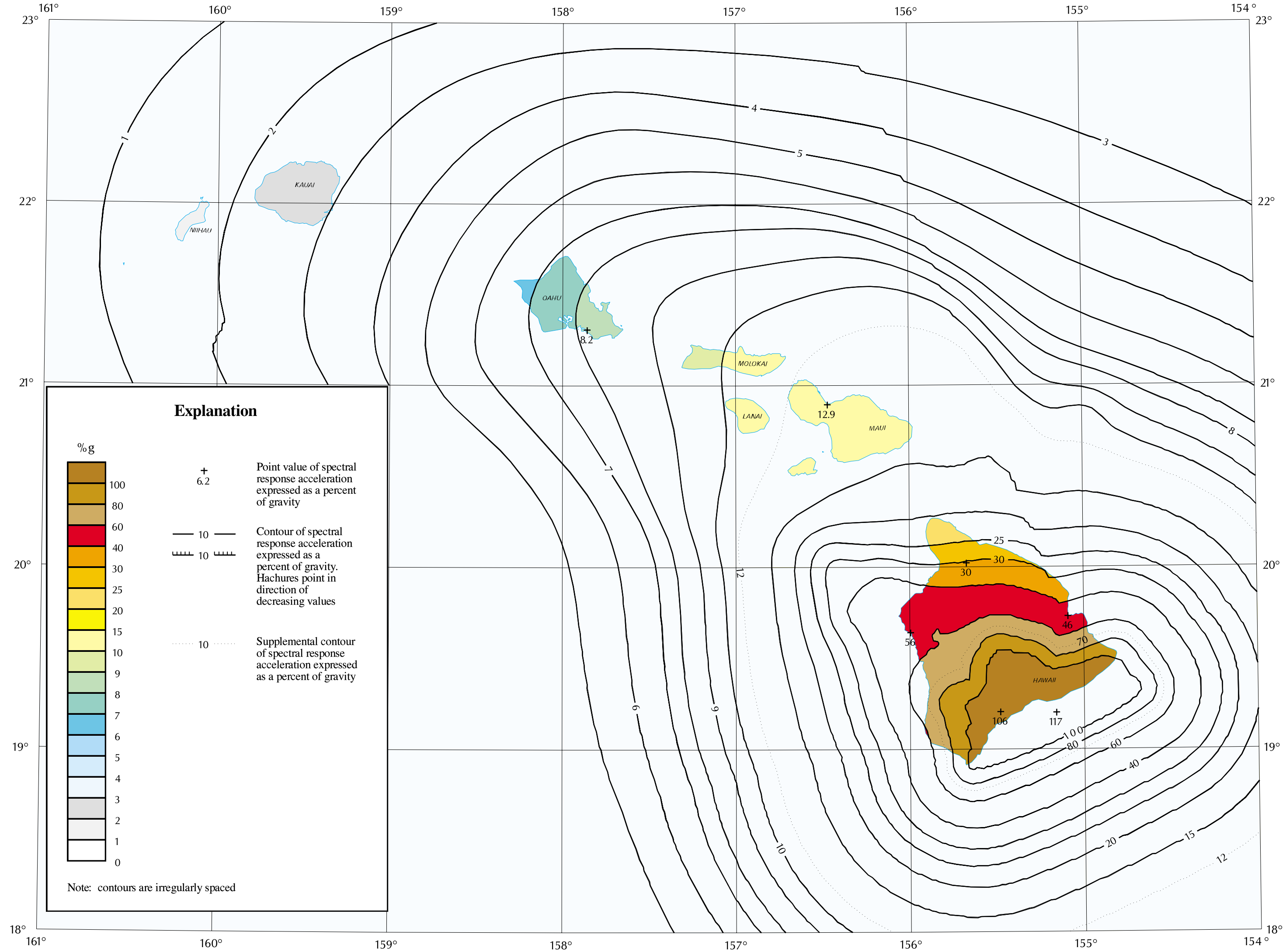
HORIZONTAL SPECTRAL RESPONSE ACCELERATION FOR 1.0 SECOND PERIOD (5% OF CRITICAL DAMPING) WITH 10% PROBABILITY OF EXCEEDANCE IN 50 YEARS
