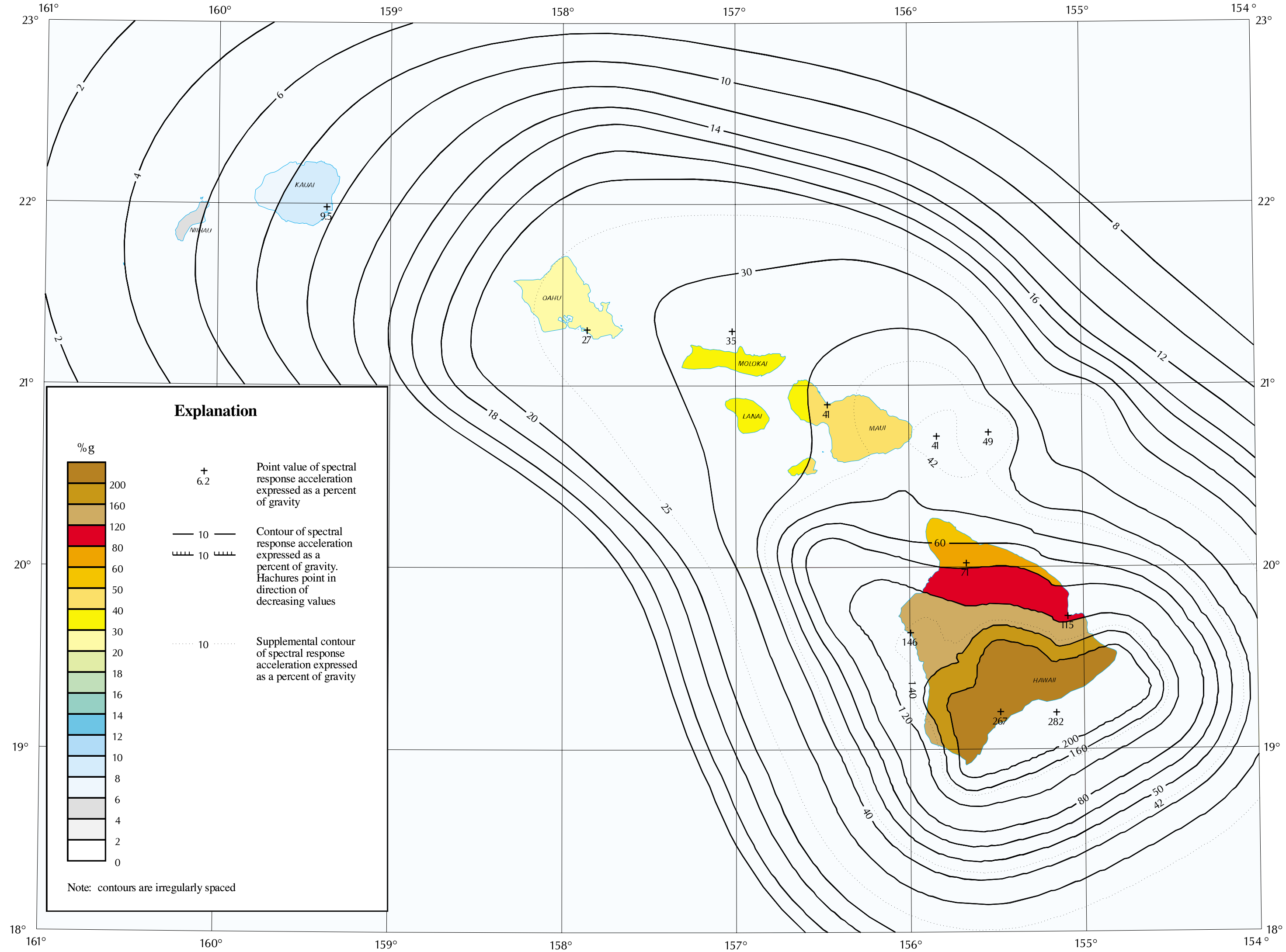
HORIZONTAL SPECTRAL RESPONSE ACCELERATION FOR 0.3 SECOND PERIOD (5% OF CRITICAL DAMPING) WITH 10% PROBABILITY OF EXCEEDANCE IN 50 YEARS
