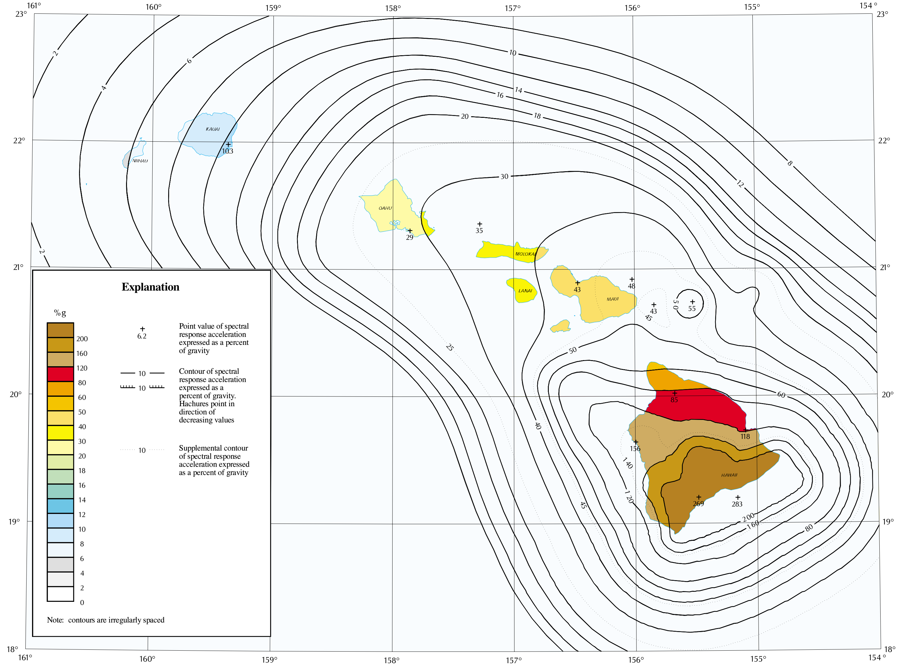
HORIZONTAL SPECTRAL RESPONSE ACCELERATION FOR 0.2 SECOND PERIOD (5% OF CRITICAL DAMPING) WITH 10% PROBABILITY OF EXCEEDANCE IN 50 YEARS
