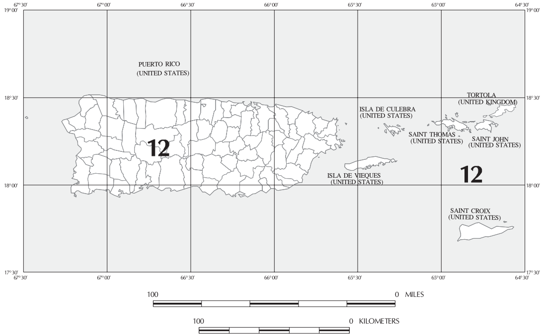
FIGURE 3.3-20 LONG-PERIOD TRANSITION PERIOD, T_L (sec), FOR PUERTO RICO, CULEBRA, VIEQUES, ST. THOMAS, ST. JOHN, AND ST. CROIX
