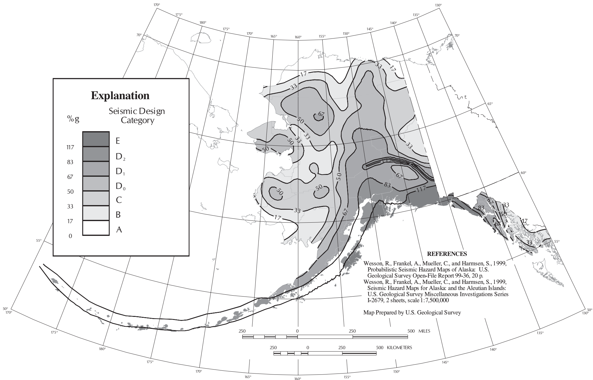
Figure R301.2(2) Alaska, Seismic Design Categories - Site Class D
