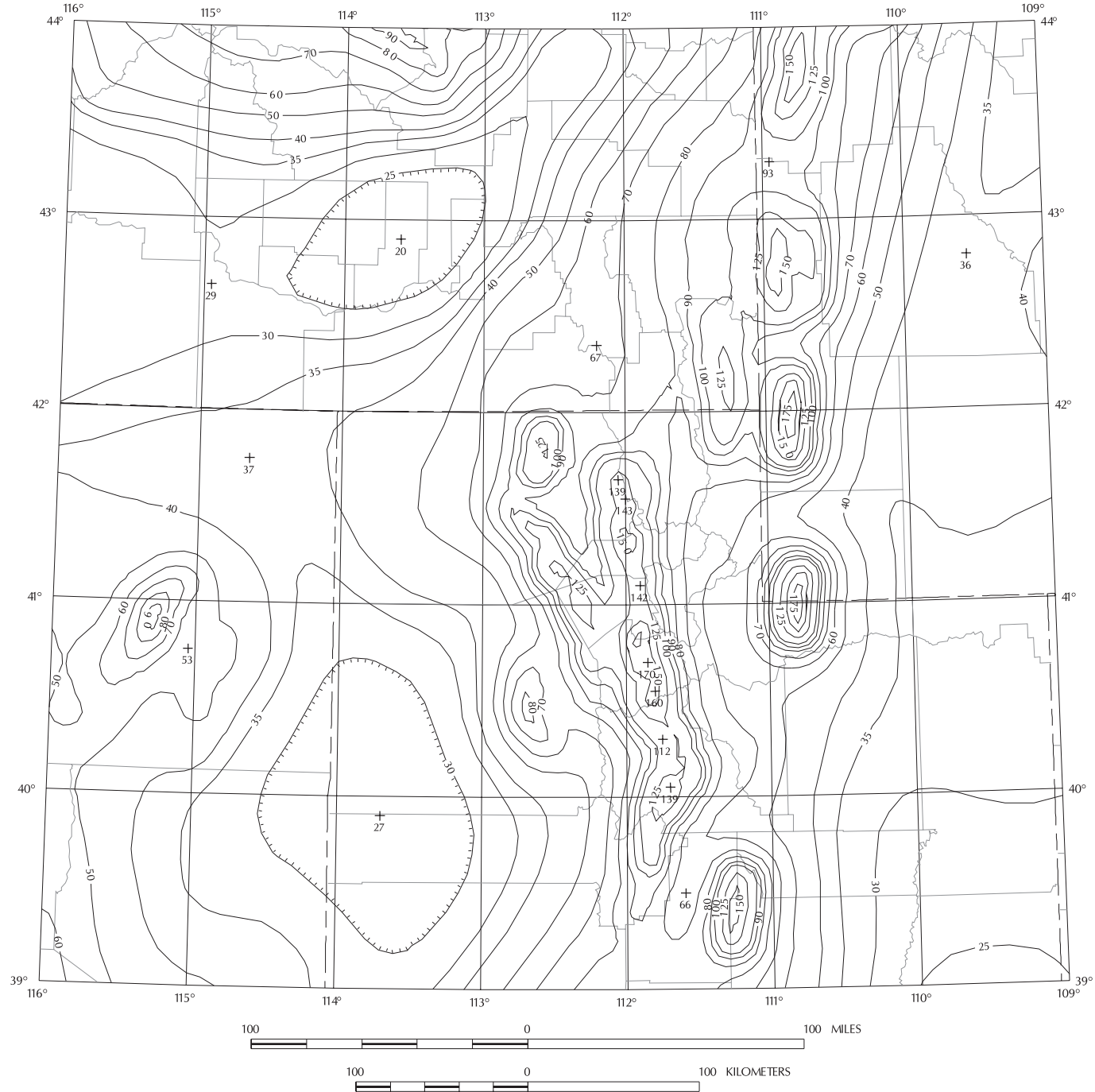
FIGURE 1613.5(5) MAXIMUM CONSIDERED EARTHQUAKE GROUND MOTION FOR REGION 2 OF 0.2 SEC SPECTRAL RESPONSE ACCELERATION (5% OF CRITICAL DAMPING), SITE CLASS B
