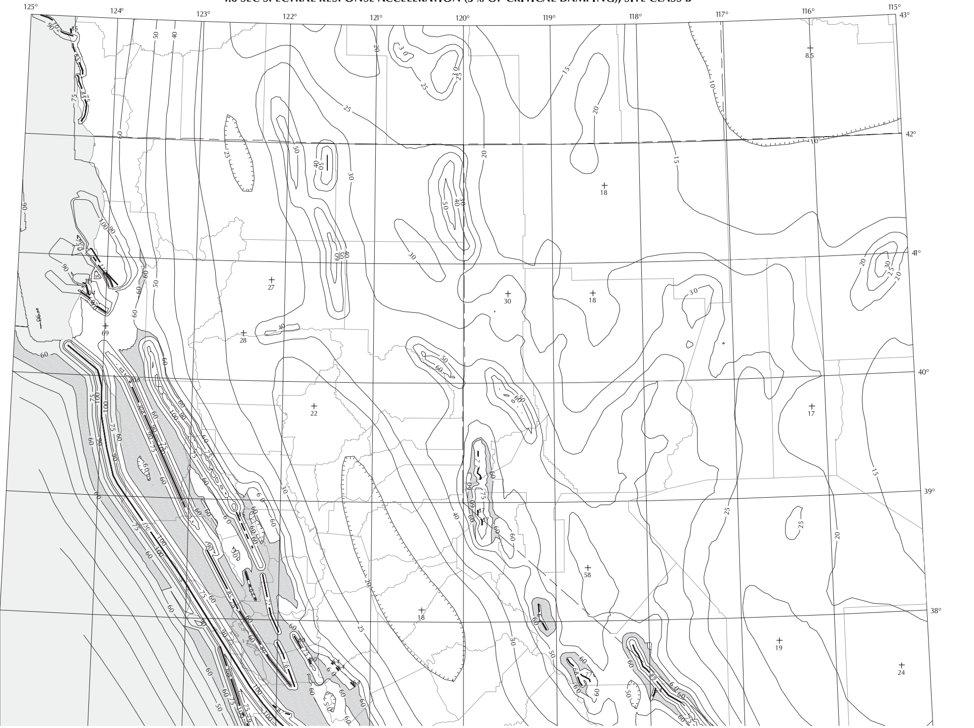
FIGURE 1613.5(4) MAXIMUM CONSIDERED EARTHQUAKE GROUND MOTION FOR REGION 1 OF 1.0 SEC SPECTRAL RESPONSE ACCELERATION (5% OF CRITICAL DAMPING), SITE CLASS B
