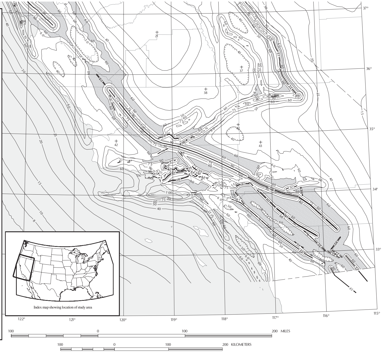
FIGURE 1613.5(4) (continued) MAXIMUM CONSIDERED EARTHQUAKE GROUND MOTION FOR REGION 1 OF 1.0 SEC SPECTRAL RESPONSE ACCELERATION (5% OF CRITICAL DAMPING), SITE CLASS B
