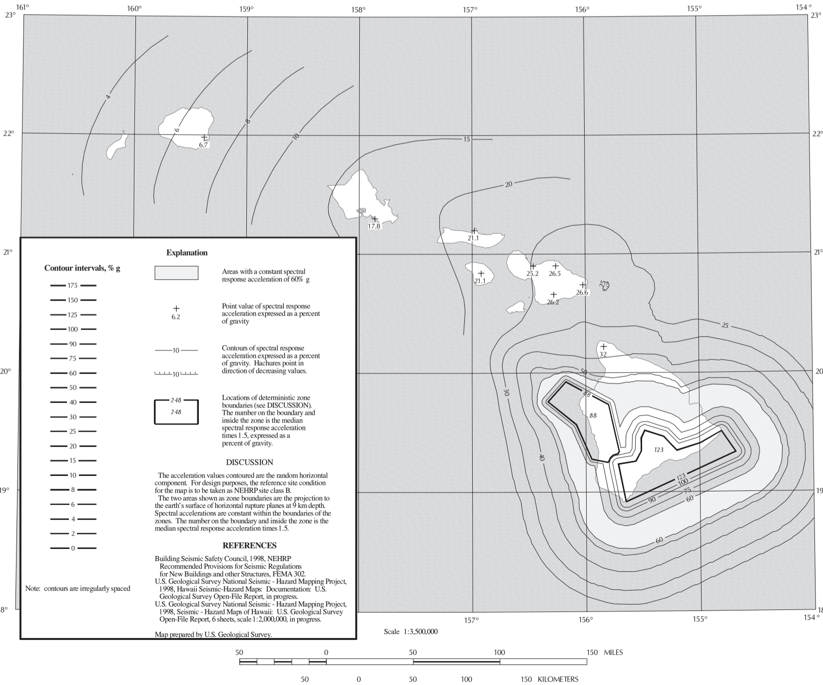
FIGURE 1615 (8)b MAXIMUM CONSIDERED EARTHQUAKE GROUND MOTION FOR HAWAII OF 1.0 SEC SPECTRAL RESPONSE ACCELERATION (5% OF CRITICAL DAMPING), SITE CLASS B
