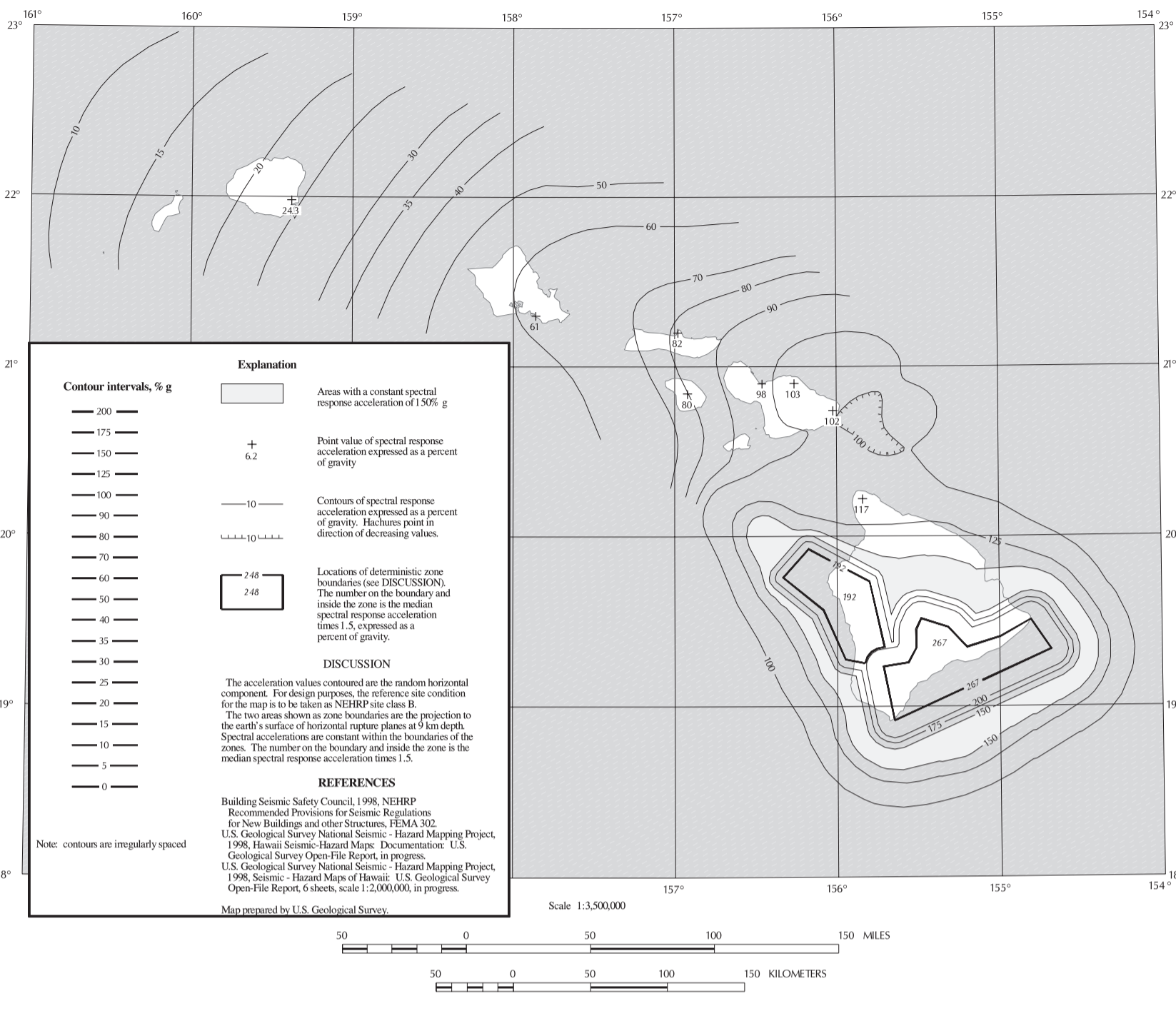
FIGURE 1615 (8)a MAXIMUM CONSIDERED EARTHQUAKE GROUND MOTION FOR HAWAII OF 0.2 SEC SPECTRAL RESPONSE ACCELERATION (5% OF CRITICAL DAMPING), SITE CLASS B
