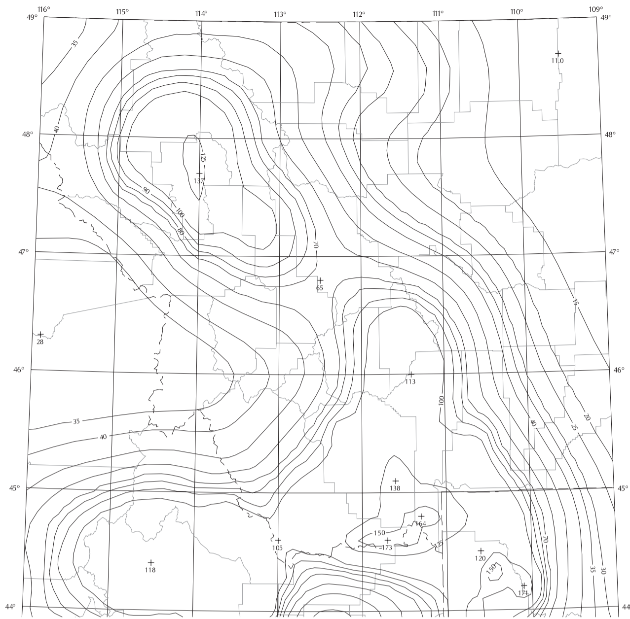
FIGURE 1615 (5) MAXIMUM CONSIDERED EARTHQUAKE GROUND MOTION FOR REGION 2 OF 0.2 SEC SPECTRAL RESPONSE ACCELERATION (5% OF CRITICAL DAMPING), SITE CLASS B
