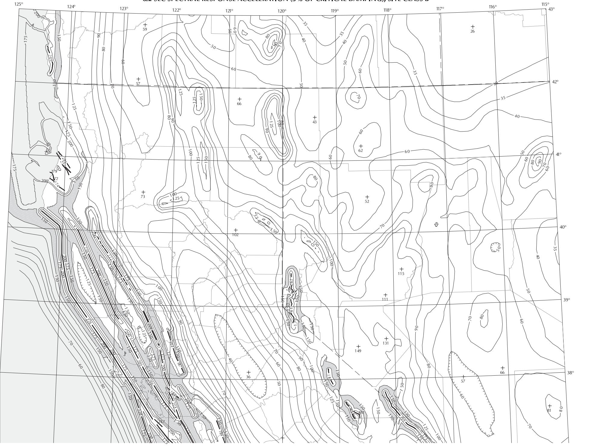
FIGURE 22-3 MAXIMUM CONSIDERED EARTHQUAKE GROUND MOTION FOR REGION 1 OF 0.2 SEC SPECTRAL RESPONSE ACCELERATION (5% OF CRITICAL DAMPING), SITE CLASS B
