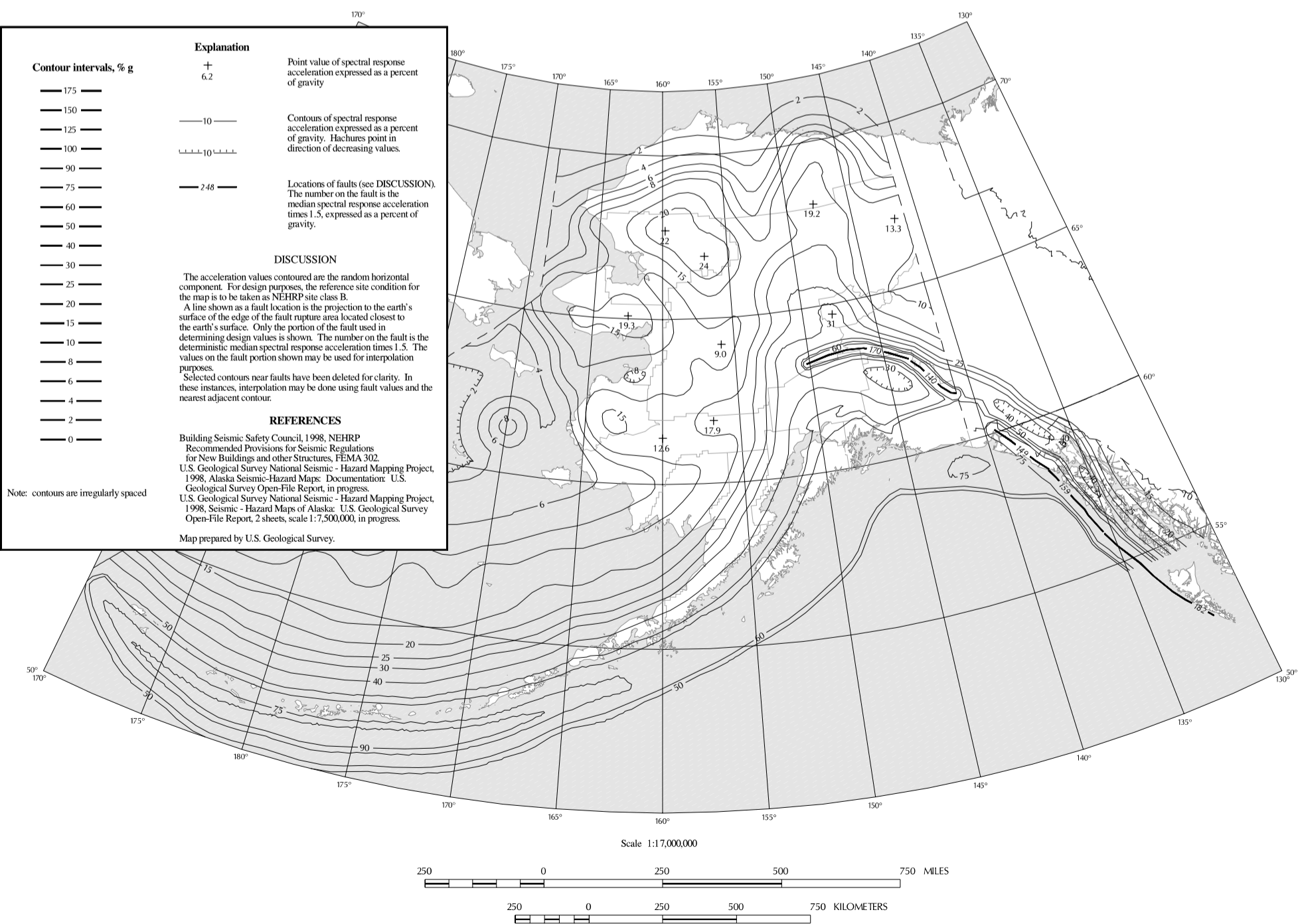
Figure 9.4.1.1 (g-2). Maximum Considered Earthquake Ground Motion for Alaska of 1.0 sec Spectral Response Acceleration (5% of Critical Damping), Site Class B.
