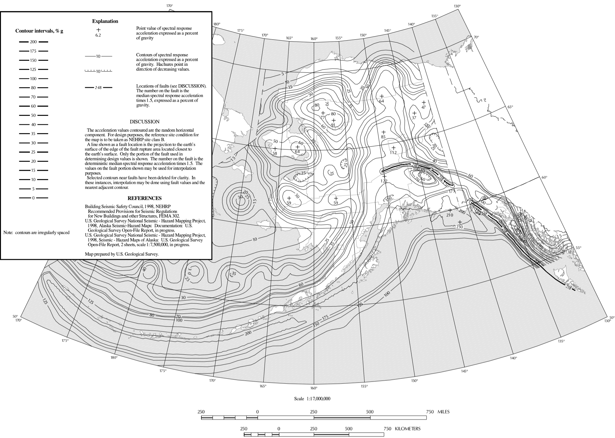
Figure 9.4.1.1 (g-1). Maximum Considered Earthquake Ground Motion for Alaska of 0.2 sec Spectral Response Acceleration (5% of Critical Damping), Site Class B.
