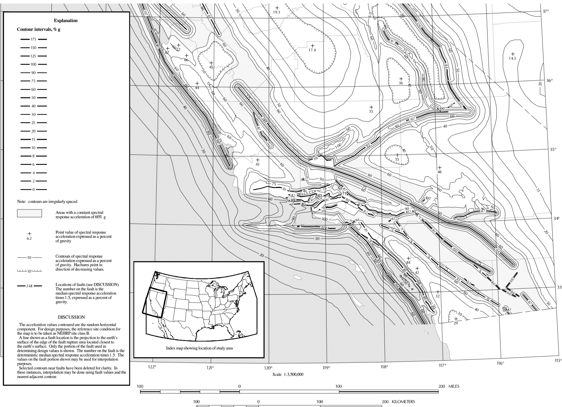
Figure 9.4.1 (d). Maximum Considered Earthquake Ground Motion for Region 1 of 1.0 sec Spectral Response Acceleration (5% of Critical Damping), Site Class B.
