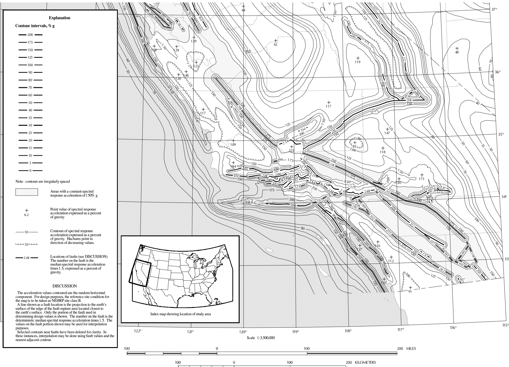
Figure 9.4.1.1 (c). Maximum Considered Earthquake Ground Motion for Region 1 of 0.2 sec Spectral Response Acceleration (5% of Critical Damping), Site Class B.
