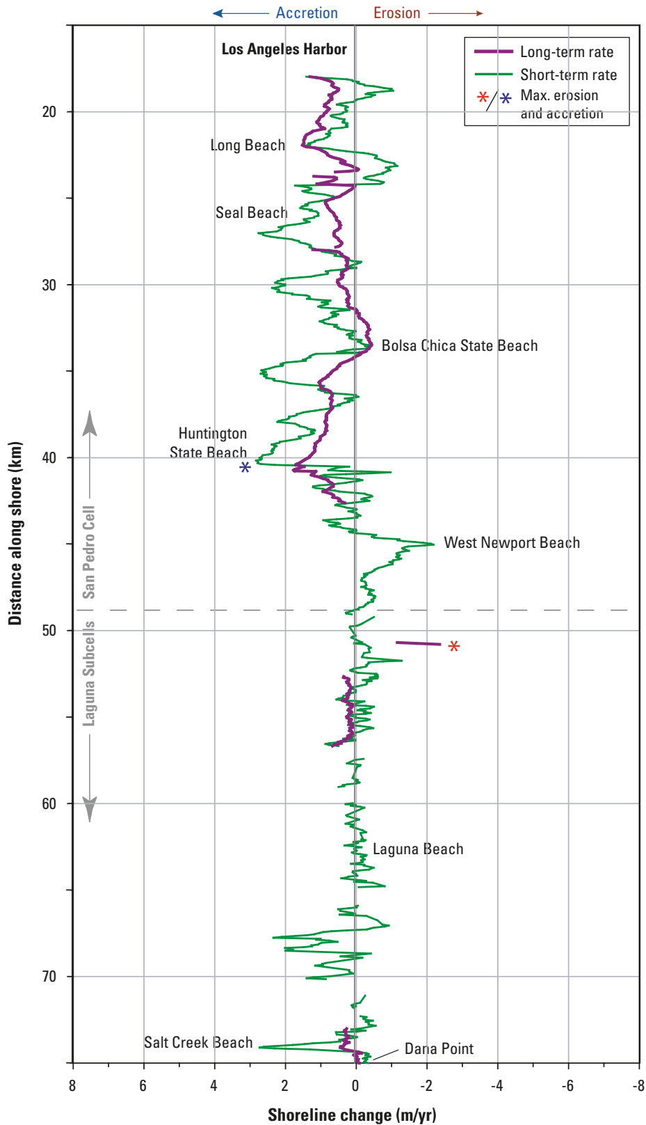
Figure 39. Shoreline change rates for the San Pedro region. The analysis extends from Los Angeles Harbor to Dana Point. The maximum long-term erosion rate was -2.4 m/yr south of Newport Bay Harbor and the maximum short-term erosion was -2.2 m/yr at Newport Beach.
