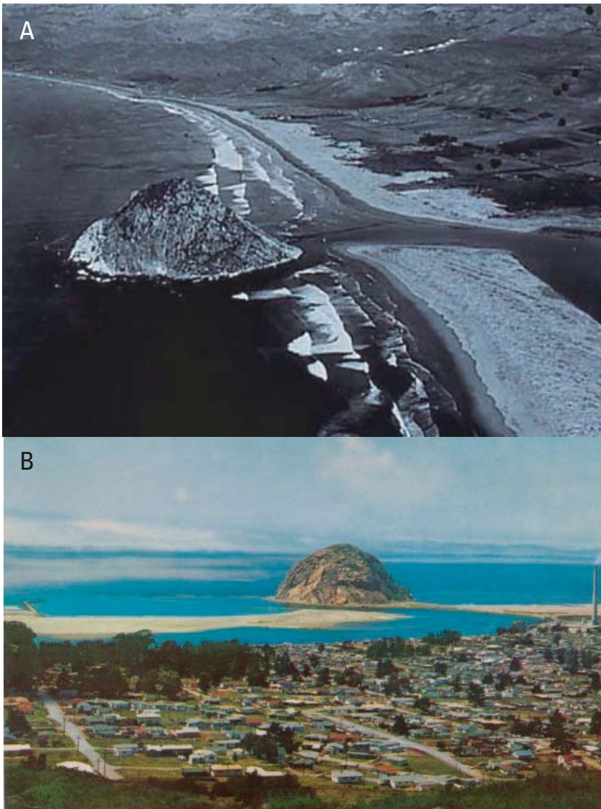
Figure 32. Development of a tombolo at Morro Rock after a causeway was built in the 1930s. Top photo was taken in 1936 just after the completion of the causeway. The postcard (lower image) is from the 1950s and shows a sandy tombolo leading out to Morro Rock (photos: http://morro-bay.com/morro-rock/ ).
