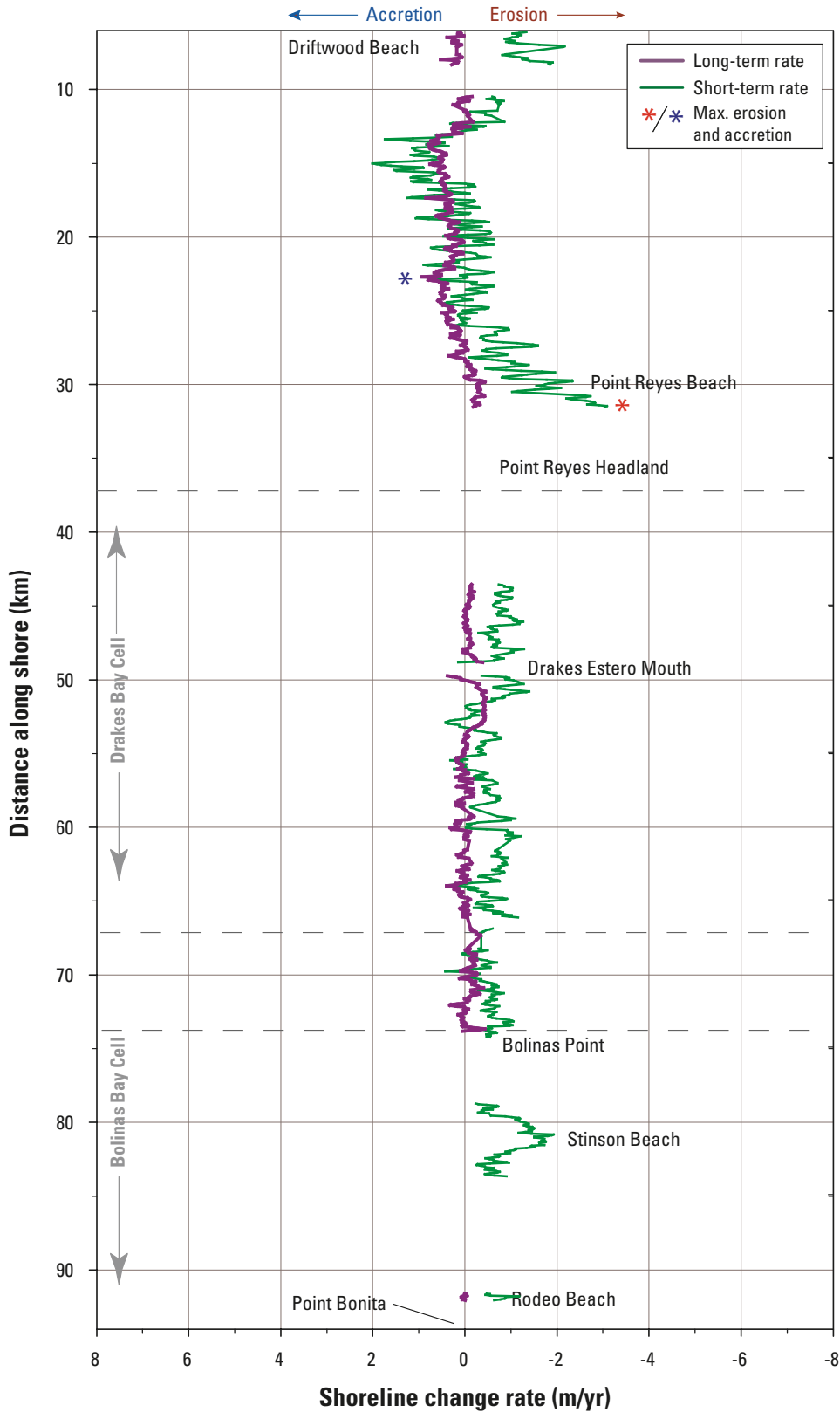
Figure 23. Shoreline change rates for the San Francisco North region. The maximum long-term erosion rate was -0.5 m/yr on Limantour Beach east of Drakes Estero; the maximum short-term erosion rate of -3.1 m/yr was measured at Point Reyes Beach just north of Point Reyes.
