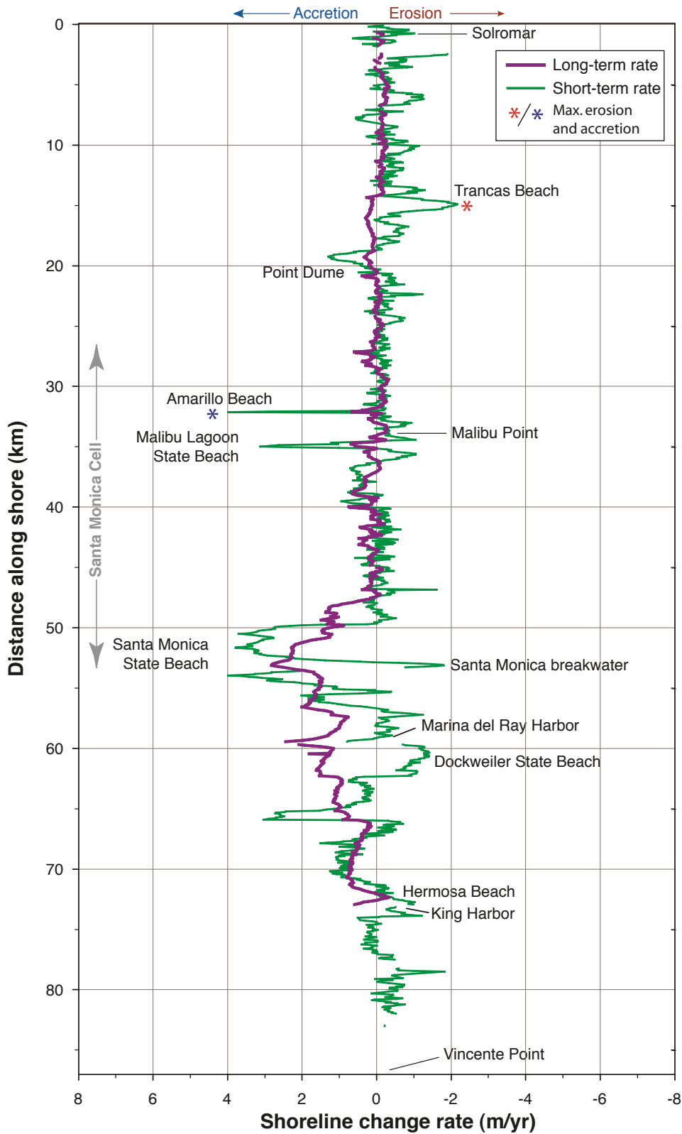
Figure 37. Shoreline change rates for the Santa Monica region. The analysis begins within the Dume subcell to the north near Solromar and extends to Vincente Point. The maximum long-term erosion rate was -0.3 m/yr at Leo Carillo State Beach and the maximum short-term erosion was -2.2 m/yr at Trancas Beach.
