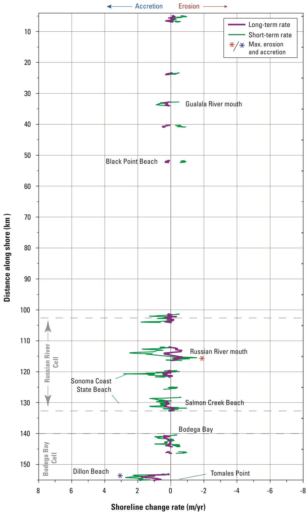
Figure 21. Shoreline change rates for the Russian River region. The maximum long-term erosion rate was -0.7 m/yr on Sonoma Coast State Beach, and the maximum short-term erosion rate of -1.6 m/yr was also measured along a remote beach along Sonoma Coast State Beach.
