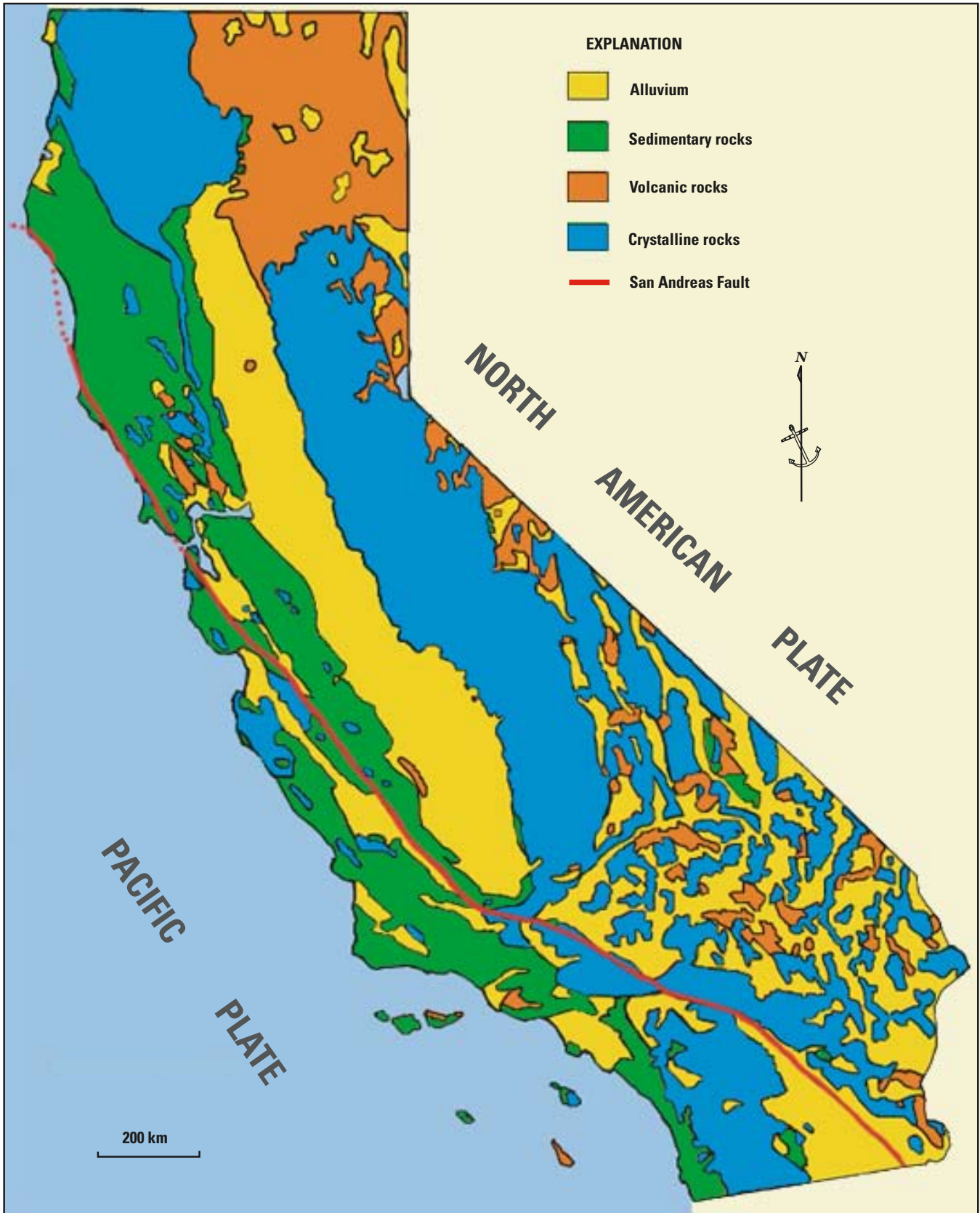
Figure 6. Simplified geologic map of California (modified from California Geological Survey generalized geologic map available on-line at: http://www.consrv.ca.gov/cgs/rghm/rgm/index.htm ).
