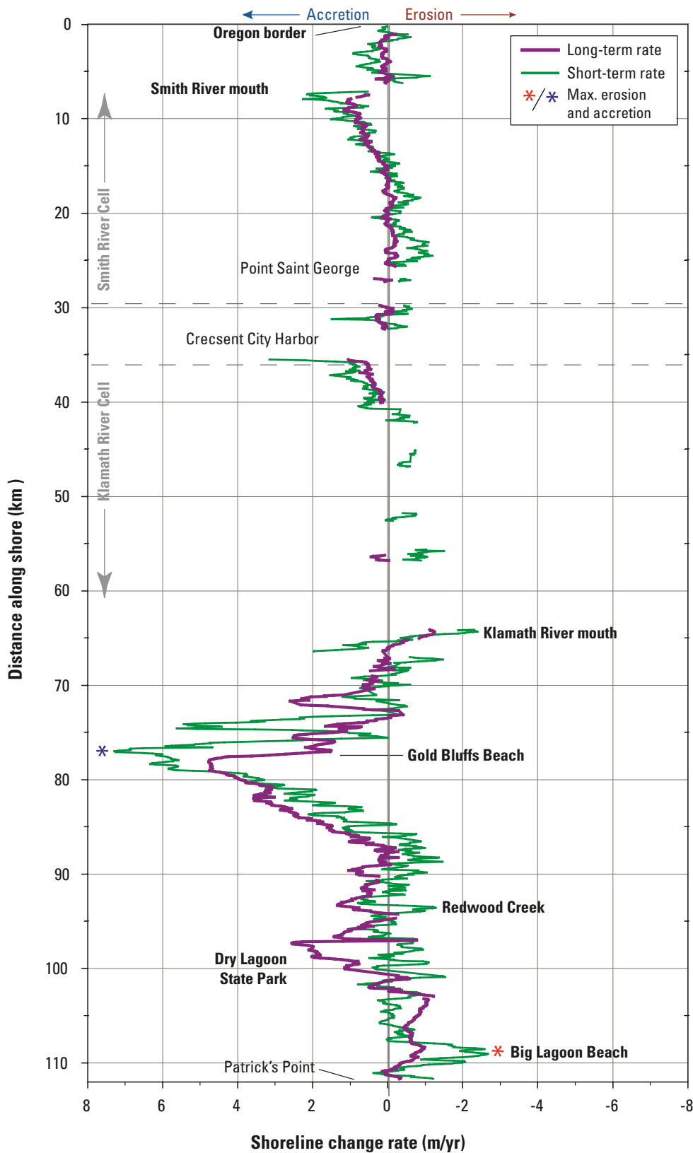
Figure 15. Shoreline change rates for the Klamath region. The maximum long-term erosion rate was -1.2 m/yr on the south side of the Klamath River mouth, and the maximum short-term erosion rate of -2.6 m/yr was measured at Big Lagoon County Park Beach.
