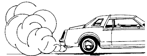
Air Pollution
