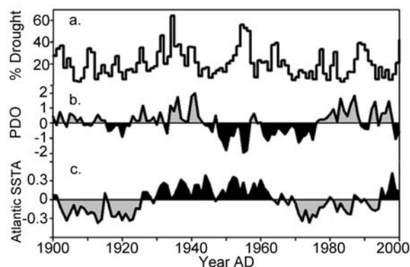
Figure 2. (a) Annual % of contiguous United States experiencing drought (PDSI < -2 ). (b) Average annual Pacific Decadal Oscillation (PDO) index [Mantua and Hare, 2002]. (c) Detrended sea surface temperature anomalies (SSTA) for the Atlantic Ocean from 0 – 70^\circ North. The Atlantic Multidecadal Oscillation (AMO) index is a ten-year running mean of this series [Enfield et al., 2001].
