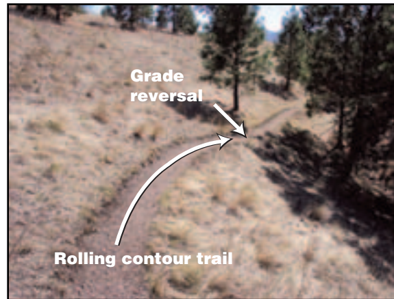
Figure 4-18—A trail with a grade reversal handles water more effectively than a trail with a waterbar. A grade reversal also requires less maintenance.
