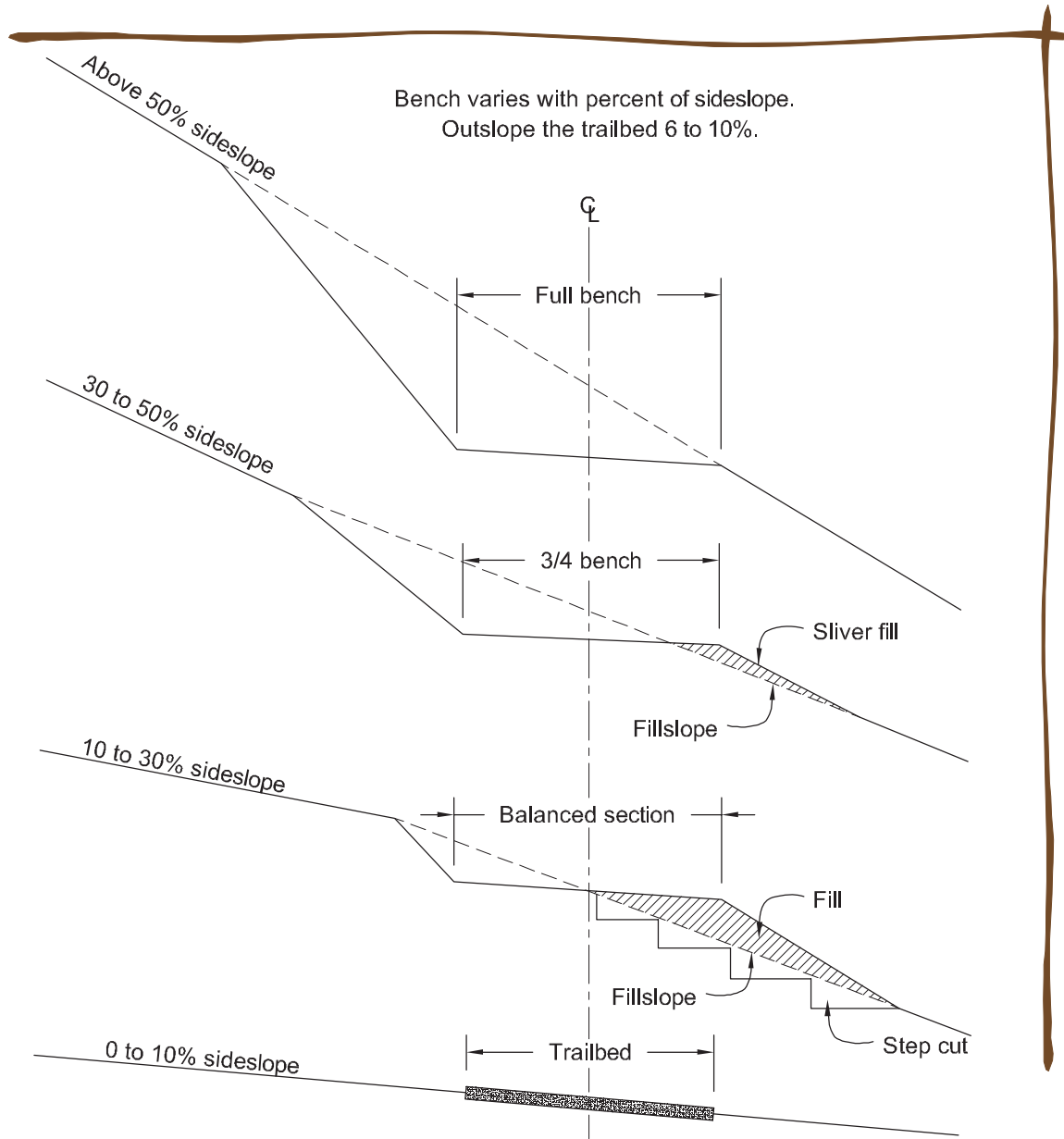
Figure 4-13—Trail typical cross sections. Full bench construction gives the fewest problems, especially on steep slopes.
