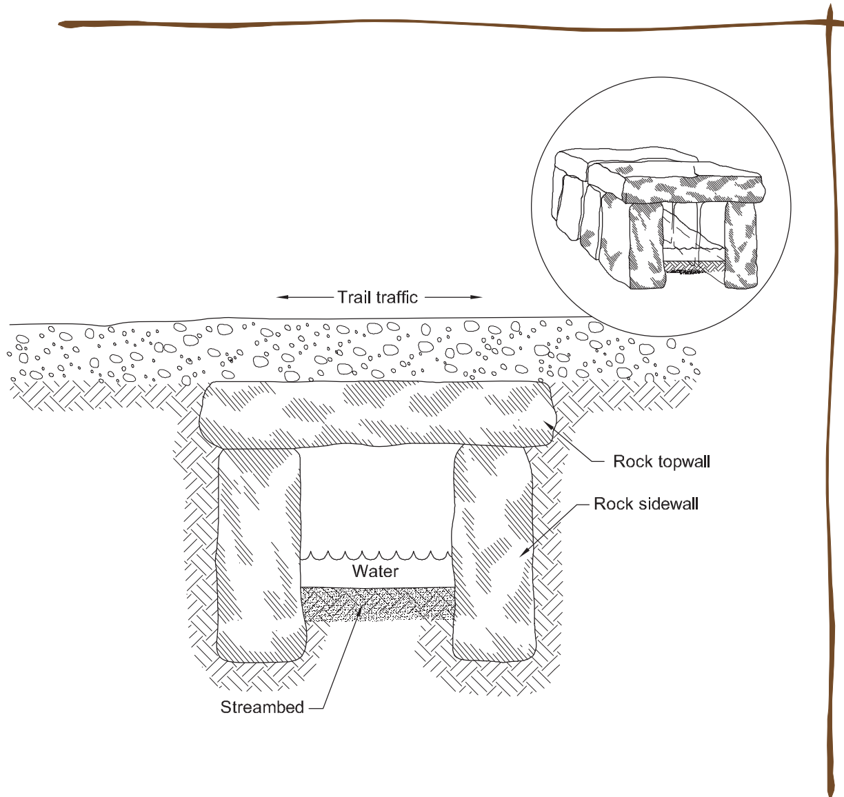
Figure 4-19—A rock culvert. Stones may also be laid along the bottom of the culvert.
