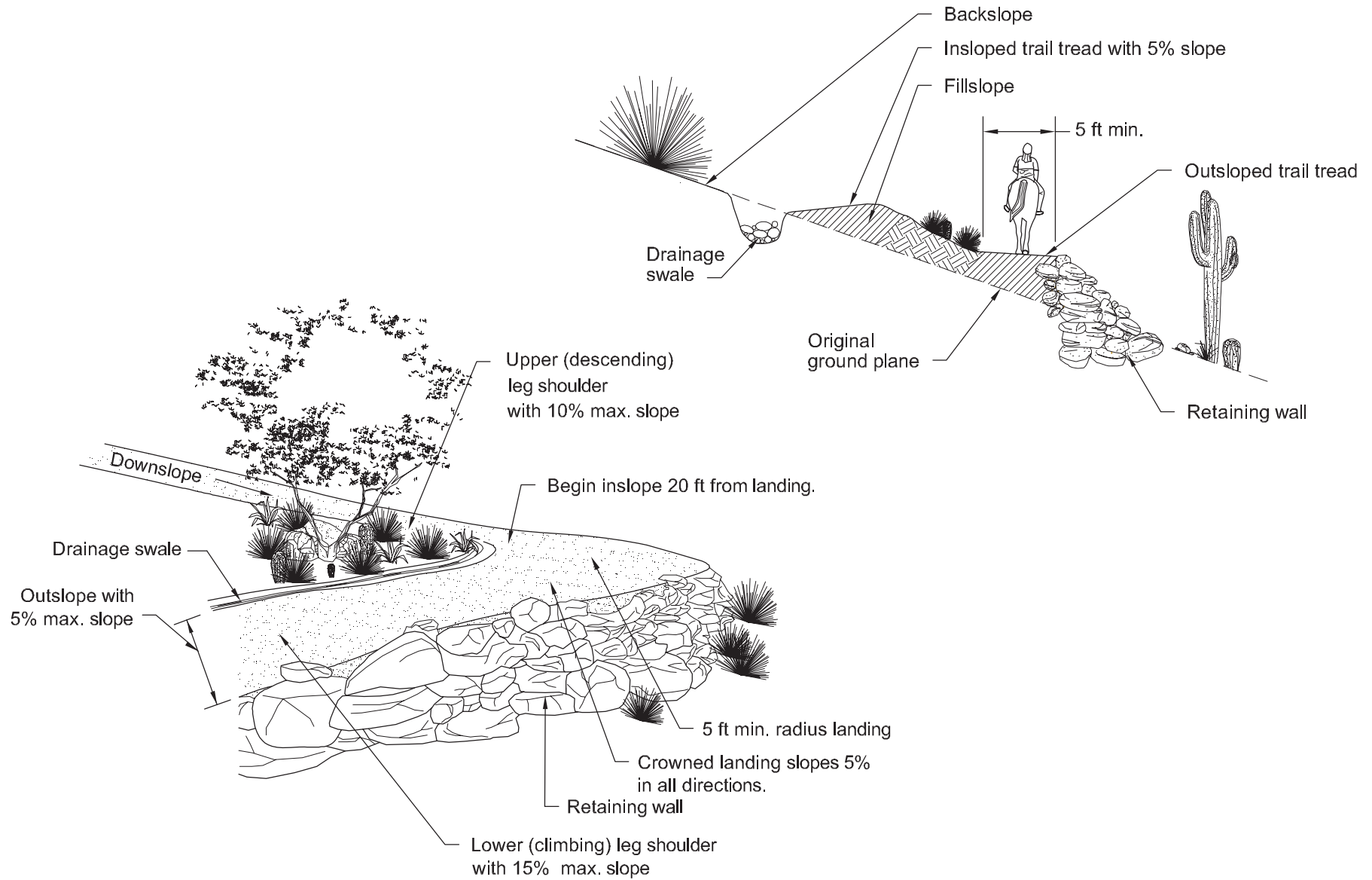
Figure 4-21—A switchback with a retaining wall.
