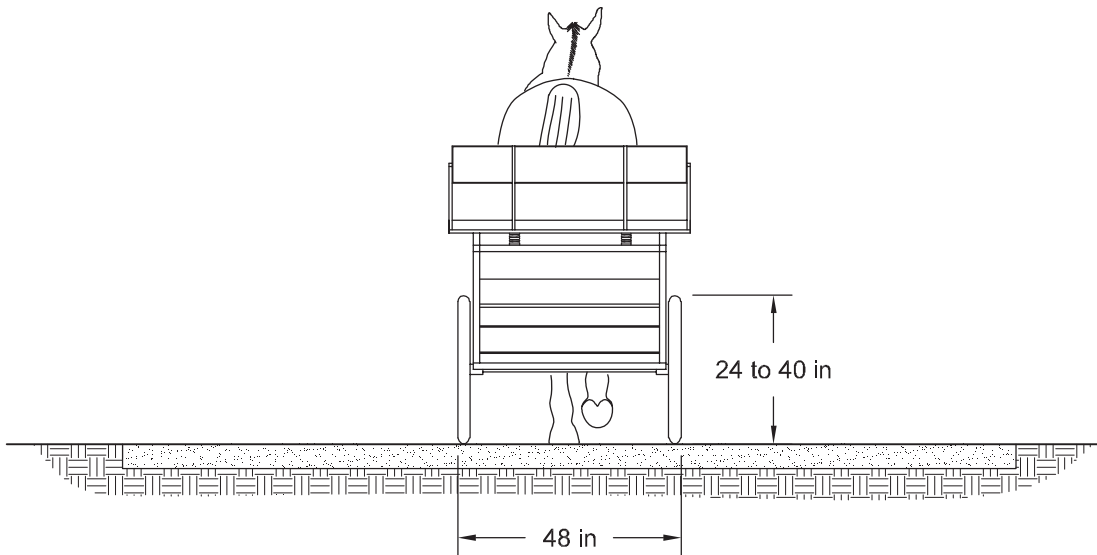
Figure 4-7—Some common dimensions for a single-horse runabout cart.
