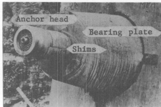
Figure 69. Wire anchorage.
