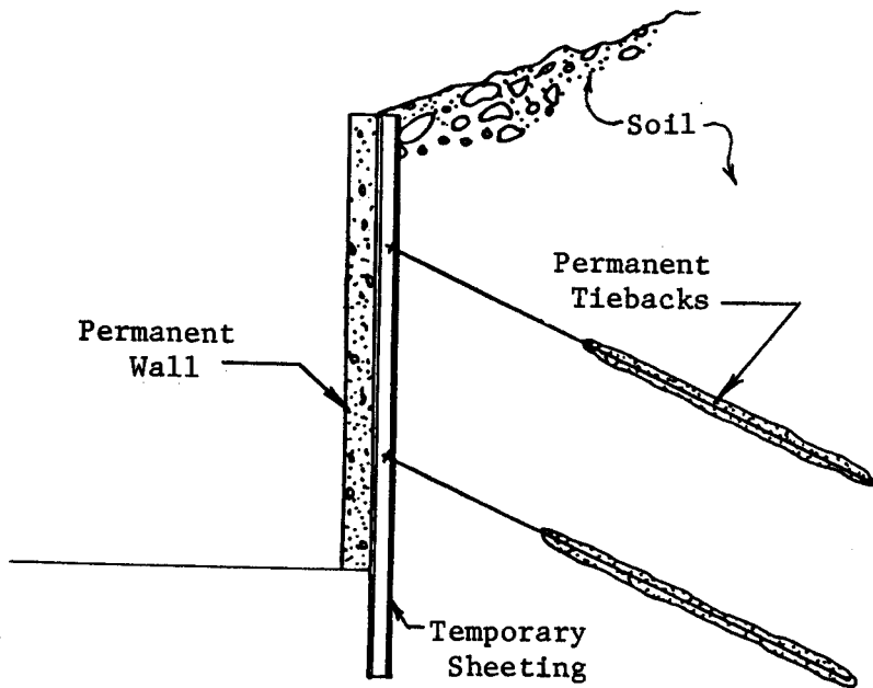
b) Permanent tiedback wall.
