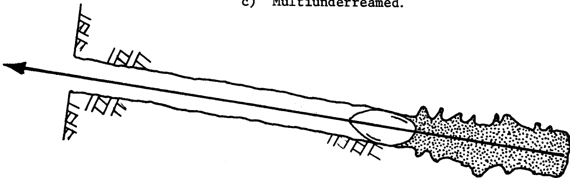
d) Postgrouted.
