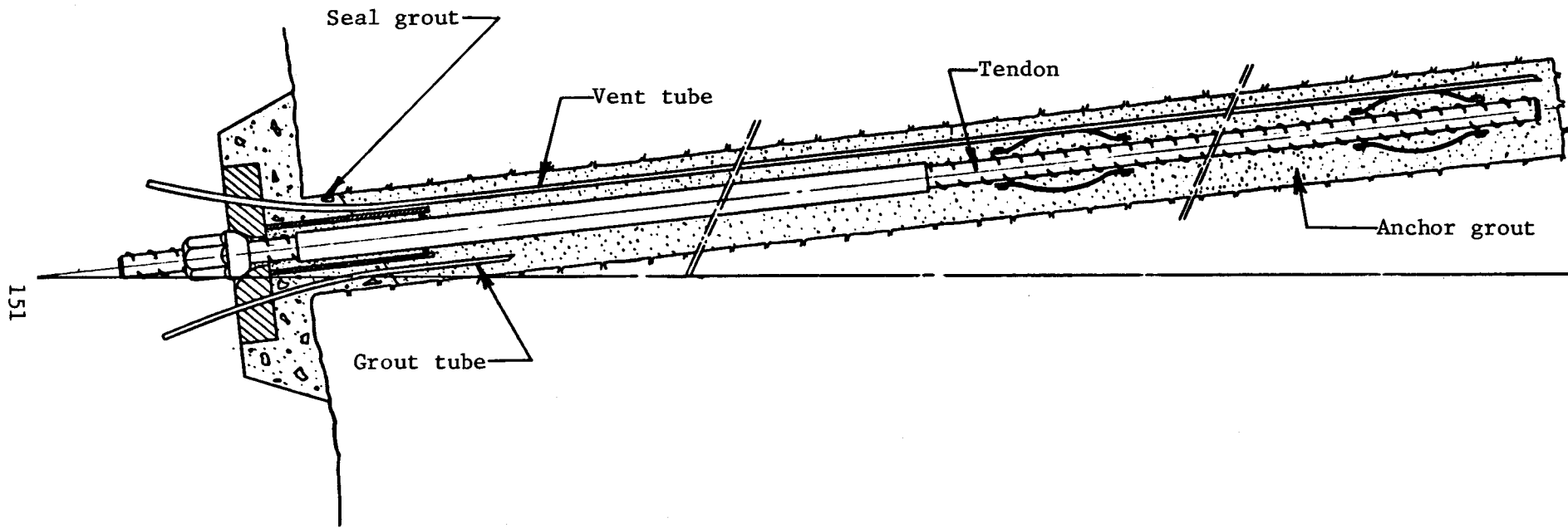
Figure 76. Grout arrangement for upward sloping rock tiebacks.
