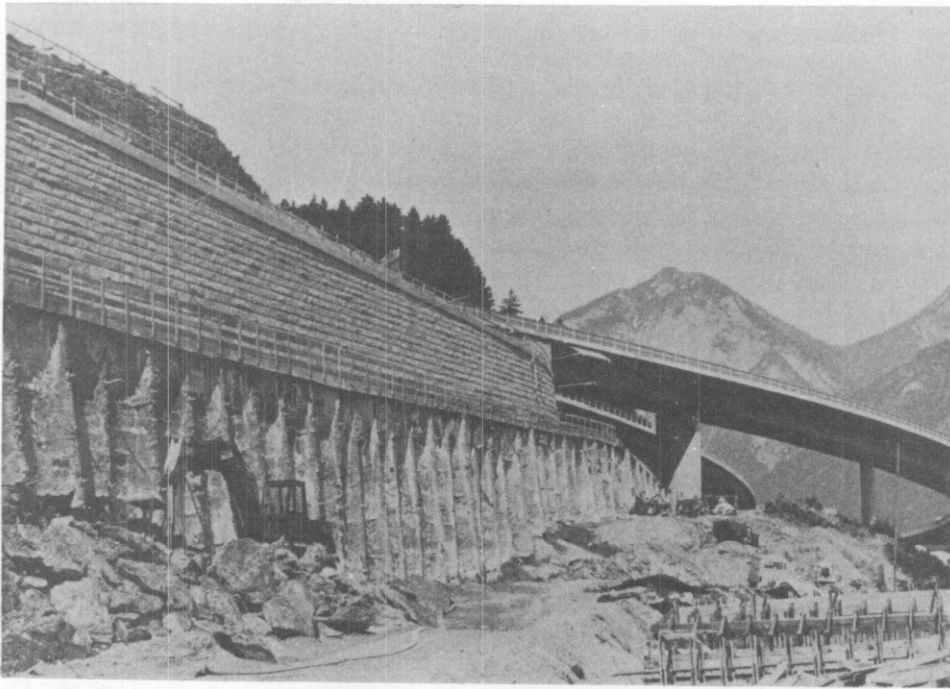
a) Tiered wall under construction (courtesy Karl Bauer).
