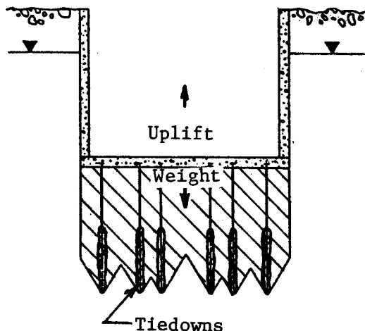
Figure 63. Determination of the total tiedown length.
