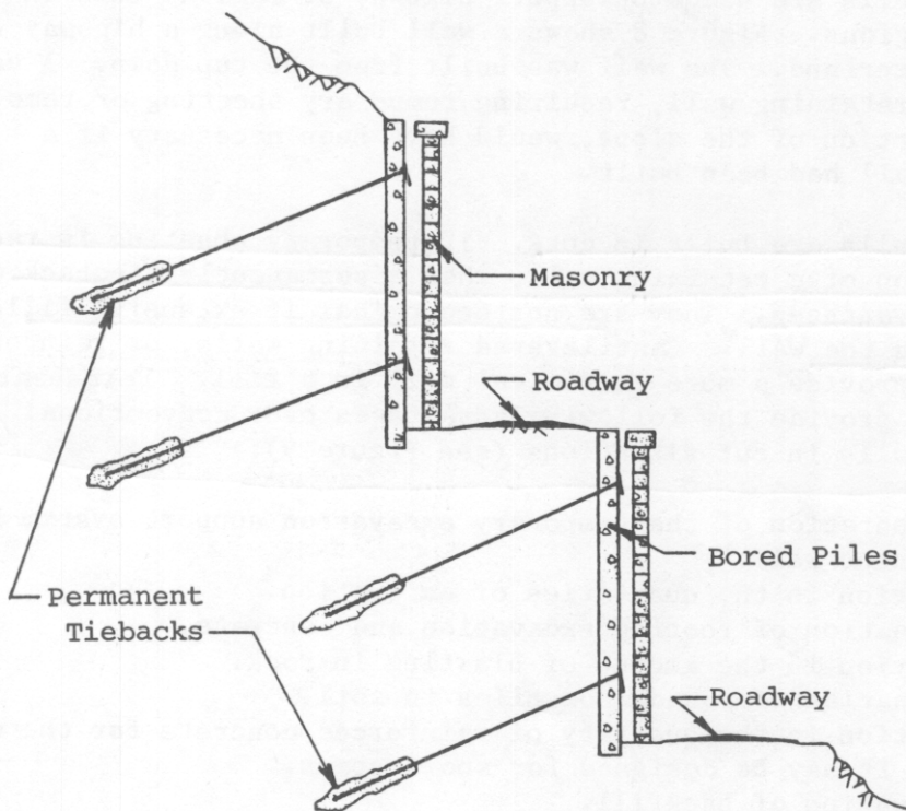
a) Tiered wall under construction (courtesy Karl Bauer).
