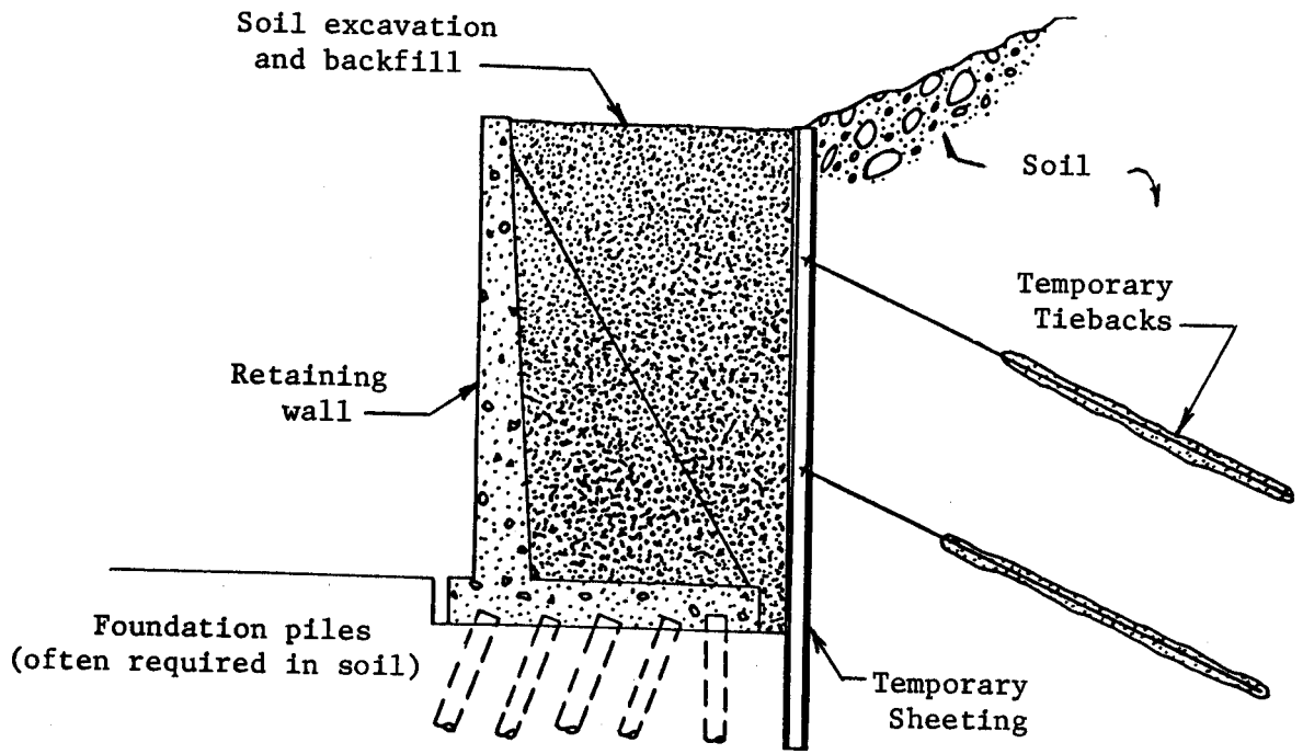
a) Conventional retaining wall .
