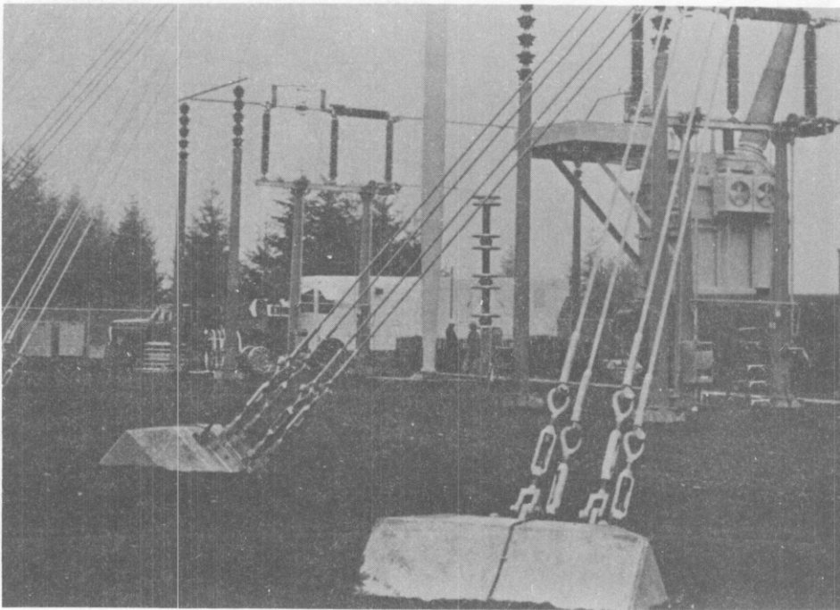
a) Completed tiedown towers (courtesy Donald B. Murphy).
