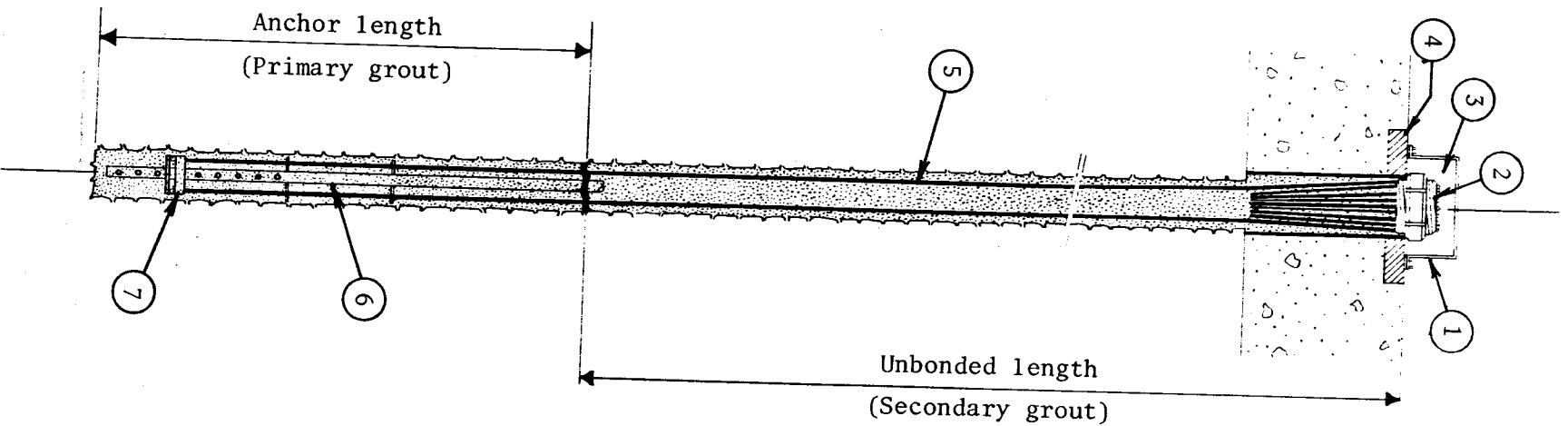
Figure 49. Primary and secondary grout used for corrosion protection of a wire tendon.
