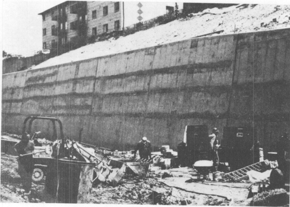
a) Permanently tiedback wall under construction.
