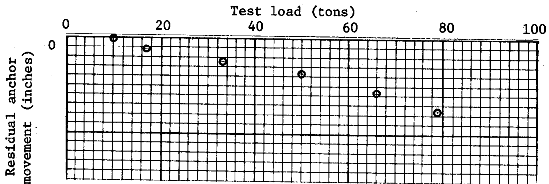
b) Residual anchor movement curve
