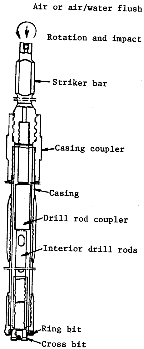
Figure 74. "Klemm" system drill string arrangement.
