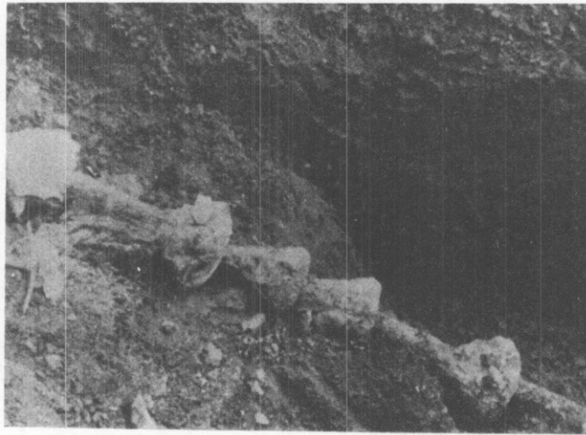
Figure 79. Multiunderreamed tieback (Courtesy Soil Mechanics Ltd.).
