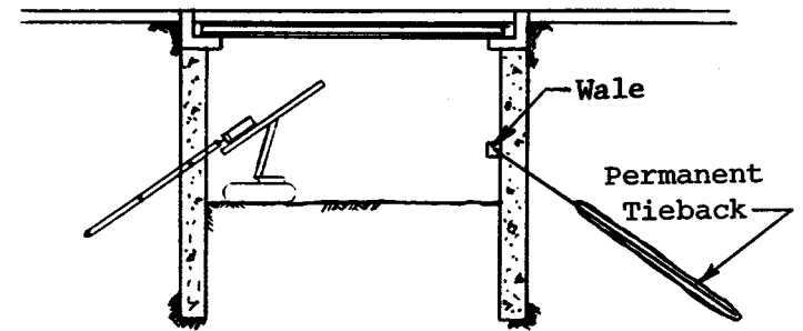
d) Excavation and tieback installation.
