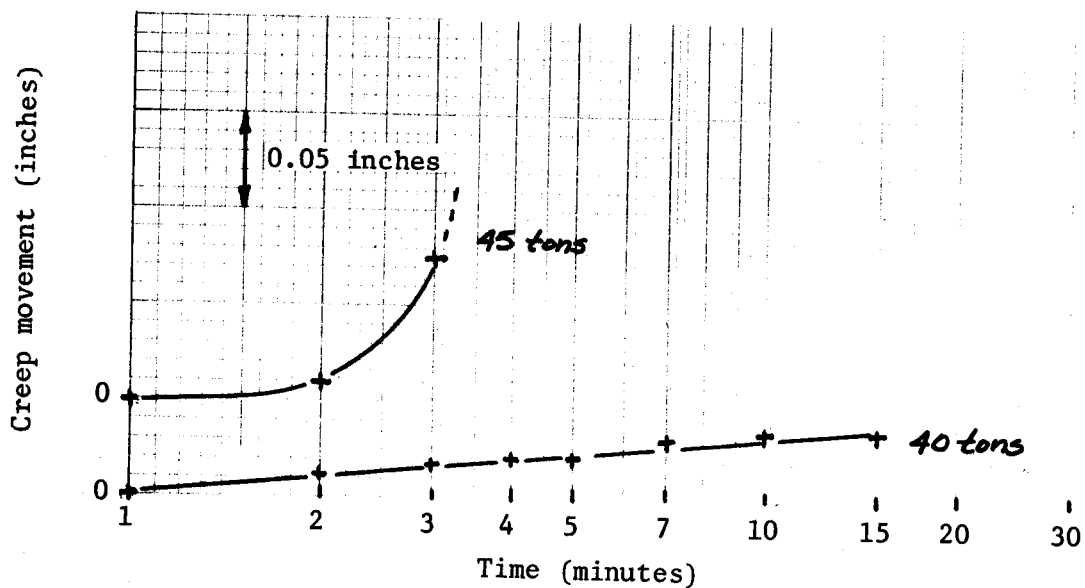
Figure 107. Creep test performed on a postgrouted tieback installed in a stiff to very stiff silty clay.
