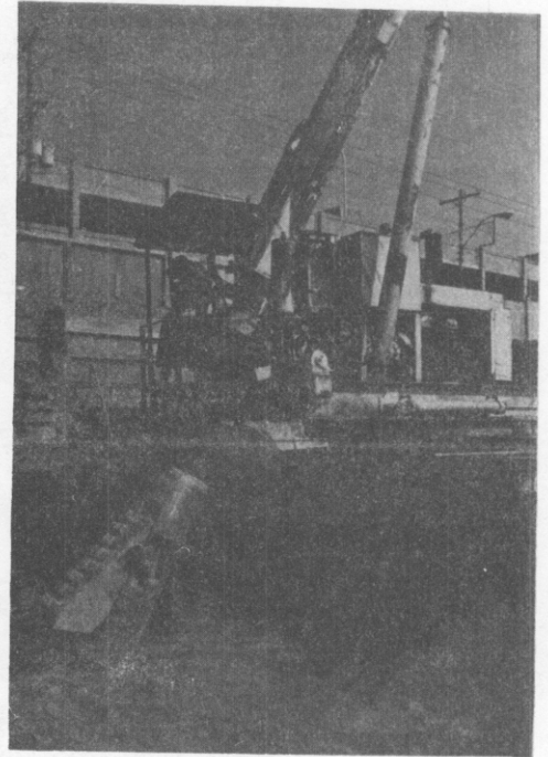
Figure 78. Caisson drill with underreaming tool.
