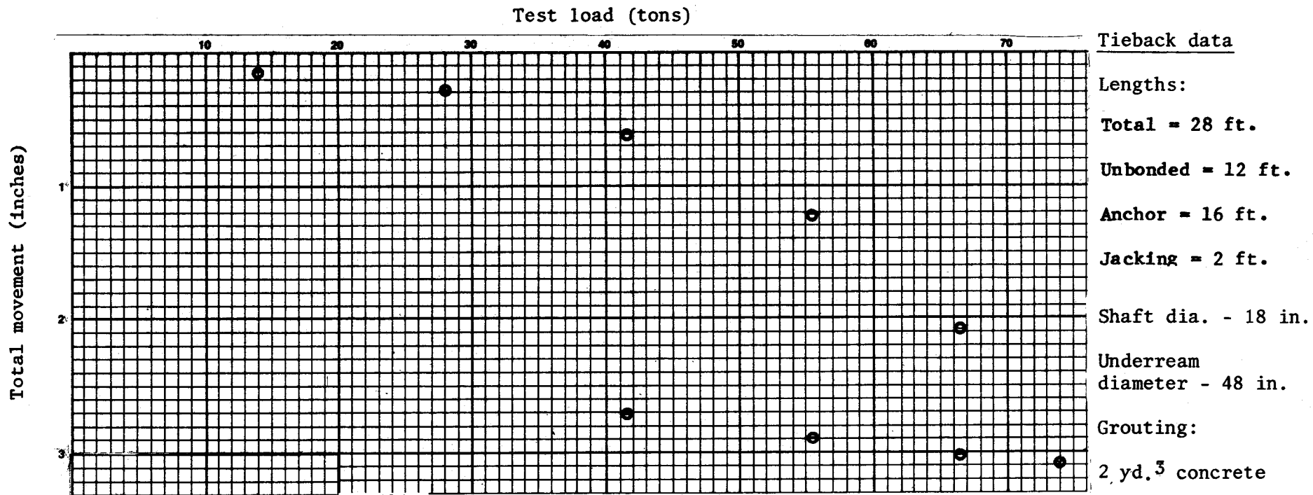
a) Total movement curve.
