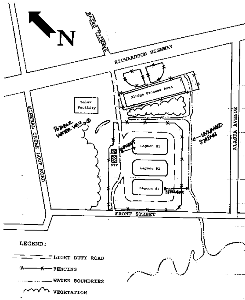
Facility Layout
