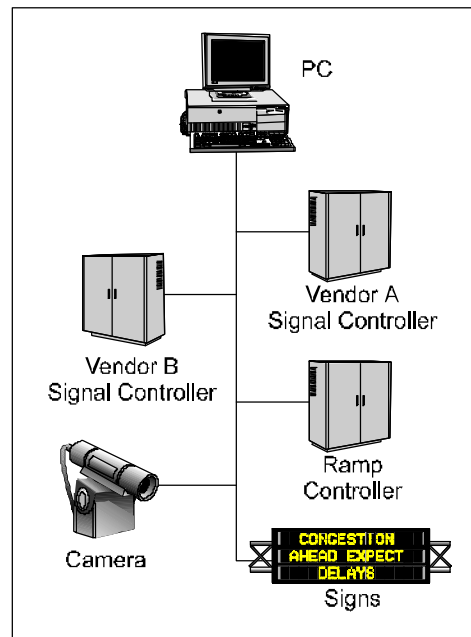
Figure 2.6-5. NTCIP Standard
