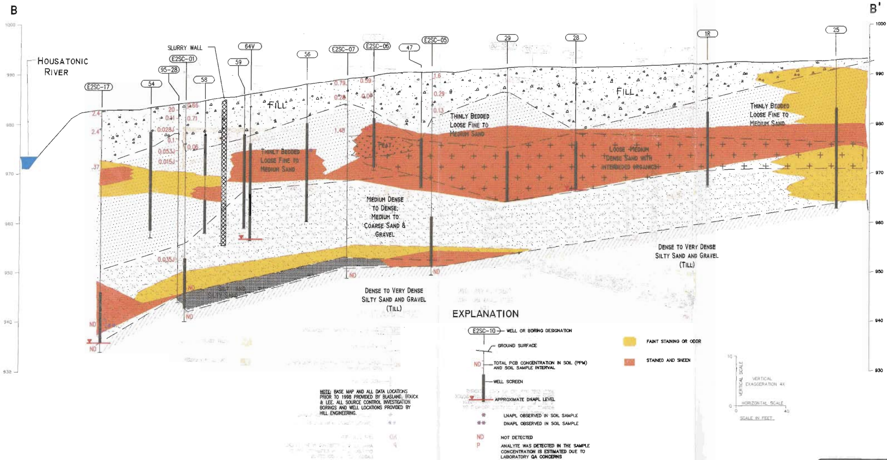
Figure 2-4 Cross-Section B-B'
