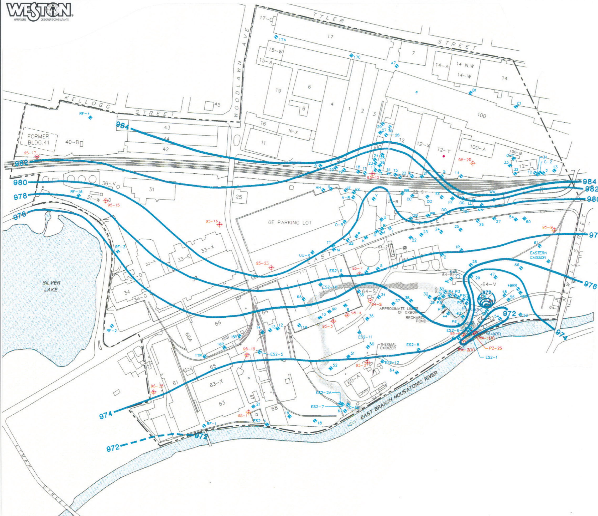
Source Area Characterization Report Pittsfield Massachusetts FIGURE 3.3.2-9 INTERPRETED GROUNDWATER CONTOUR MAP, EAST STREET AREA 2-1996
