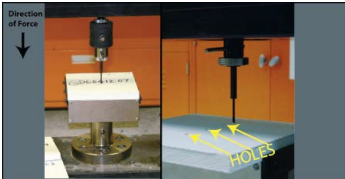
Figure 7.1 Photograph – Gypsum Wallboard Coupon Test
