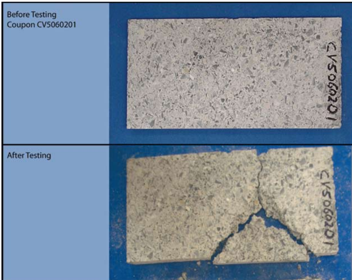
Figure 10.2 Representative Concrete Coupons Before and After Testing
