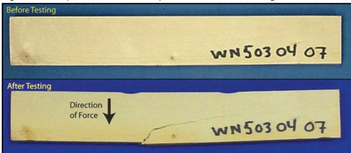
Figure 11.2 Representative Wood Coupon Before and After Testing
