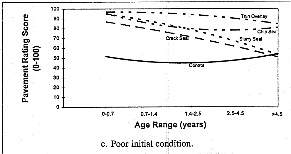
Figure 14. Pavement rating score (PRS) vs. age range by treatment type and initial condition for the wet-no freeze environmental zone, post-construction data only.
