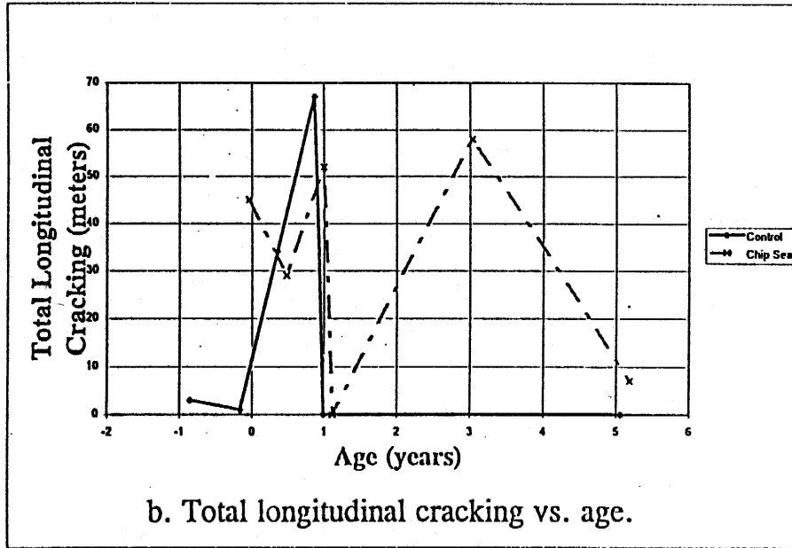
Figure 7. Example of how PRS reduces data variability for Utah site 49B300.
