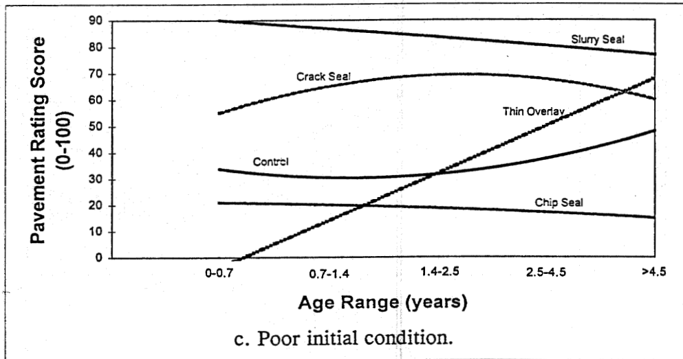
Figure 12. Pavement rating score (PRS) vs. age range by treatment type and initial condition for the dry-no freeze environmental zone, post-construction data only.
