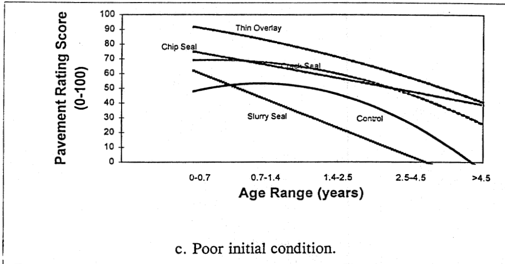
Figure 11. Pavement rating score (PRS) vs. age range by treatment type and initial condition for the dry-freeze environmental zone, post-construction data only.
