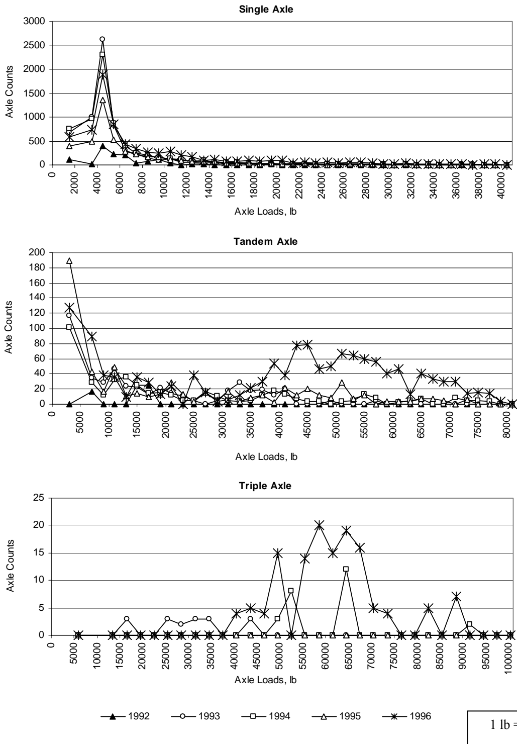
Figure 16. Rejection of all available annual axle load spectra.
