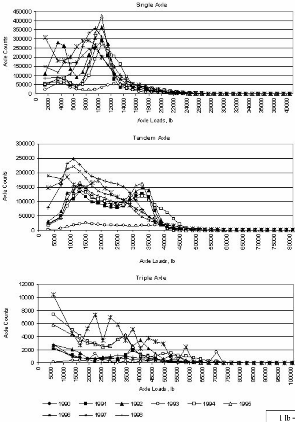
Figure 14. Use of the mean of 1991, 1992, and 1995 annual axle load spectra to obtain base annual spectrum.
