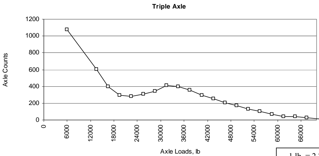
Figure 9. Average annual load spectrum for site 285805.
