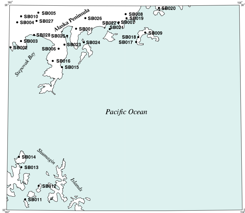
Distribution of mineral occurrences in the Stepovak Bay 1:250,000-scale quadrangle, Alaska
