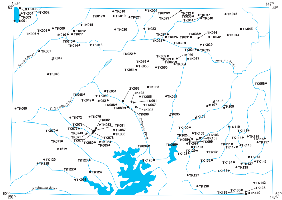
Distribution of mineral occurrences in the Talkeetna Mountains 1:250,000-scale quadrangle, Alaska
