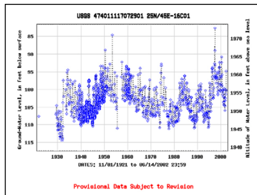
Figure 3. Greenacres, WA. One of the longest records of ground-water levels in the country.
