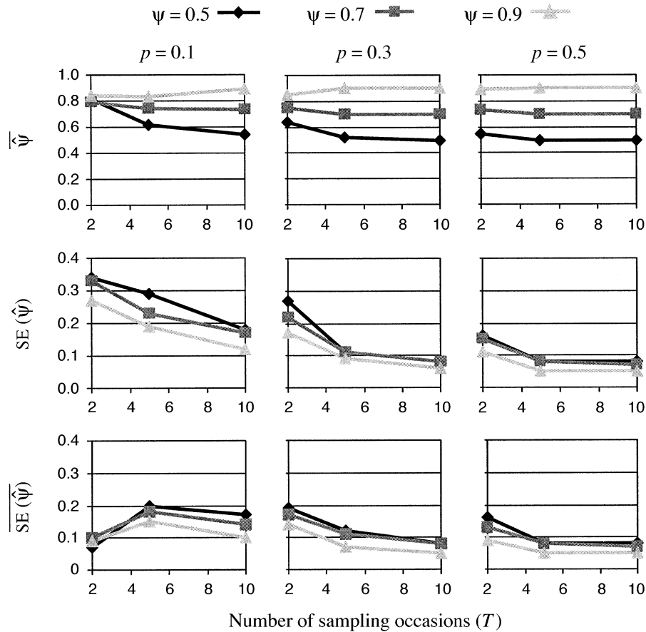
FIG. 1. Results of the 500 simulated sets of data for N = 40 , with no missing values. Indicated are the average value of \hat{\psi} , \bar{\hat{\psi}} ; the replication-based estimate of the true standard error of \hat{\psi} , SE(\hat{\psi}) ; and the average estimate of the standard error obtained from 200 nonparametric bootstrap samples, SE(\hat{\psi}) , for various levels of T , p , and \psi .
