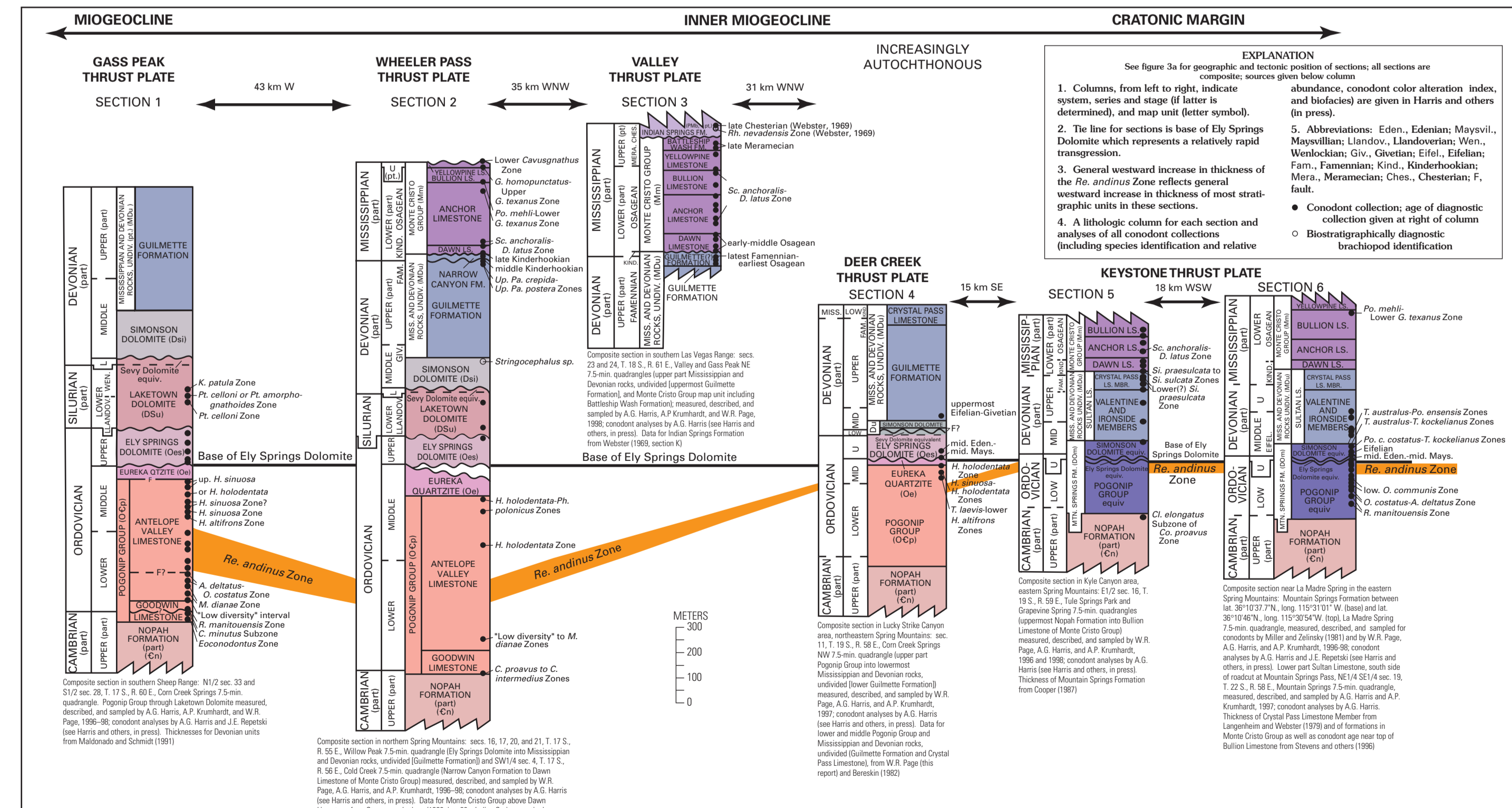
Figure 2. Correlation of selected Paleozoic units in major thrust plates, Las Vegas 30' x 60' quadrangle.
