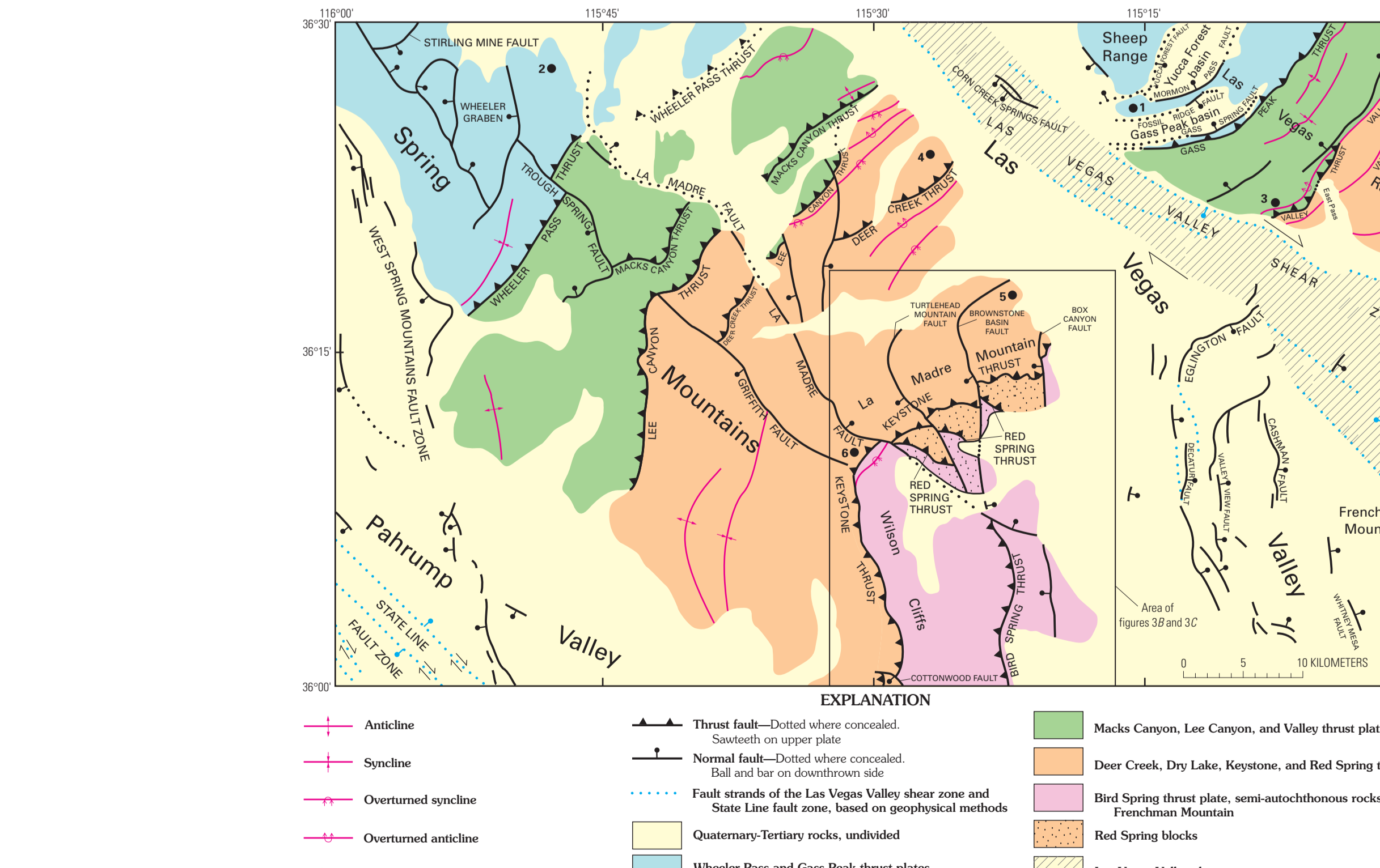
Figure 3A. Map showing major structures in the Las Vegas 30' x 60' quadrangle.
