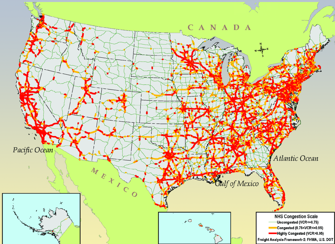
FIGURE 3-9. PEAK-PERIOD CONGESTION ON THE NATIONAL HIGHWAY SYSTEM: 2035
