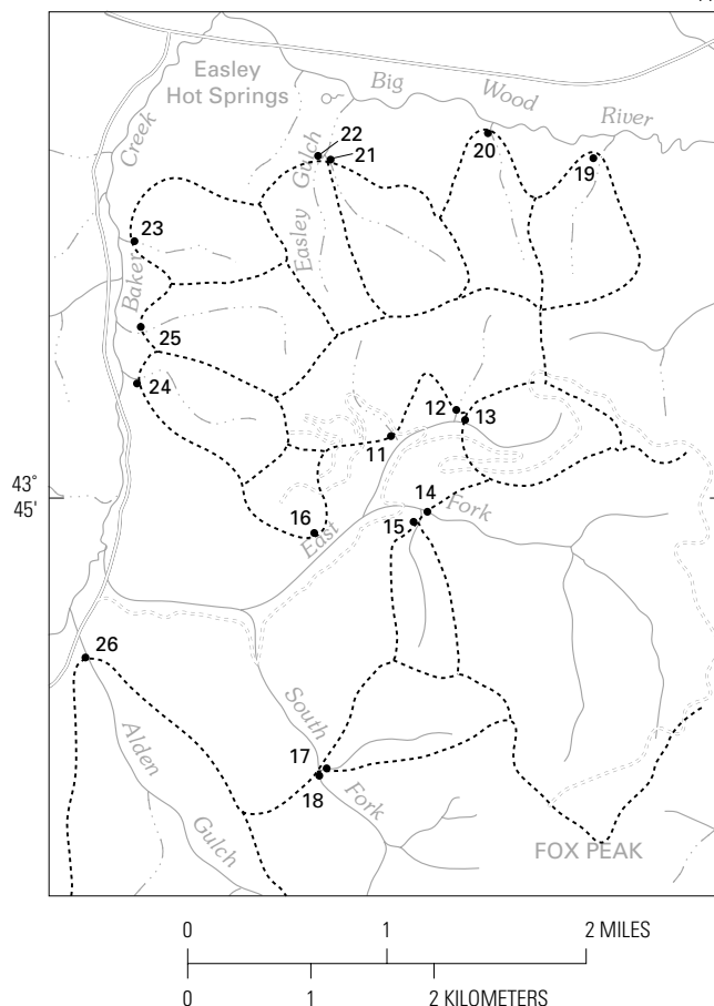
Figure 5. Stream-sediment, heavy mineral concentrate, and aquatic moss sample localities, Baker Creek study area, Idaho. Dashed lines indicate approximate limits of drainage basins associated with sample localities.
