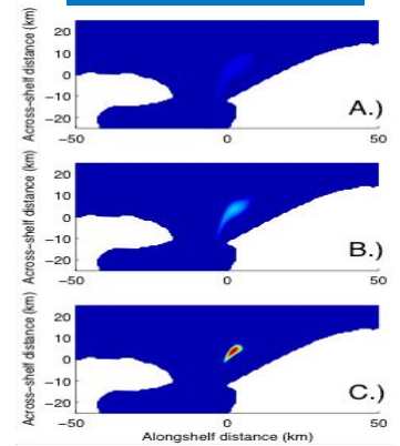
*Larvae concentrations from three simulations in which a 3 km patch of larvae is introduced into the flow field. The panels represent the patch 10 days after formation assuming that larvae are passive (A), swim at 1 cm/s (B), and swim at 2 cm/s (C). This highlights that larval swimming can significantly affect patch dynamics.
