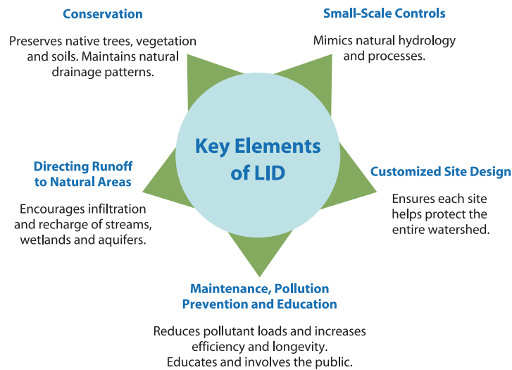
Figure 6. Low-Impact Development
