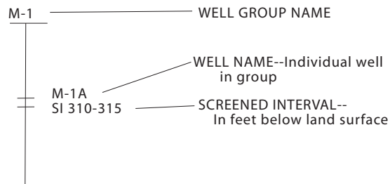
Mesquite hydrologic section (modified from Nickerson, 1986, fig. 16).
