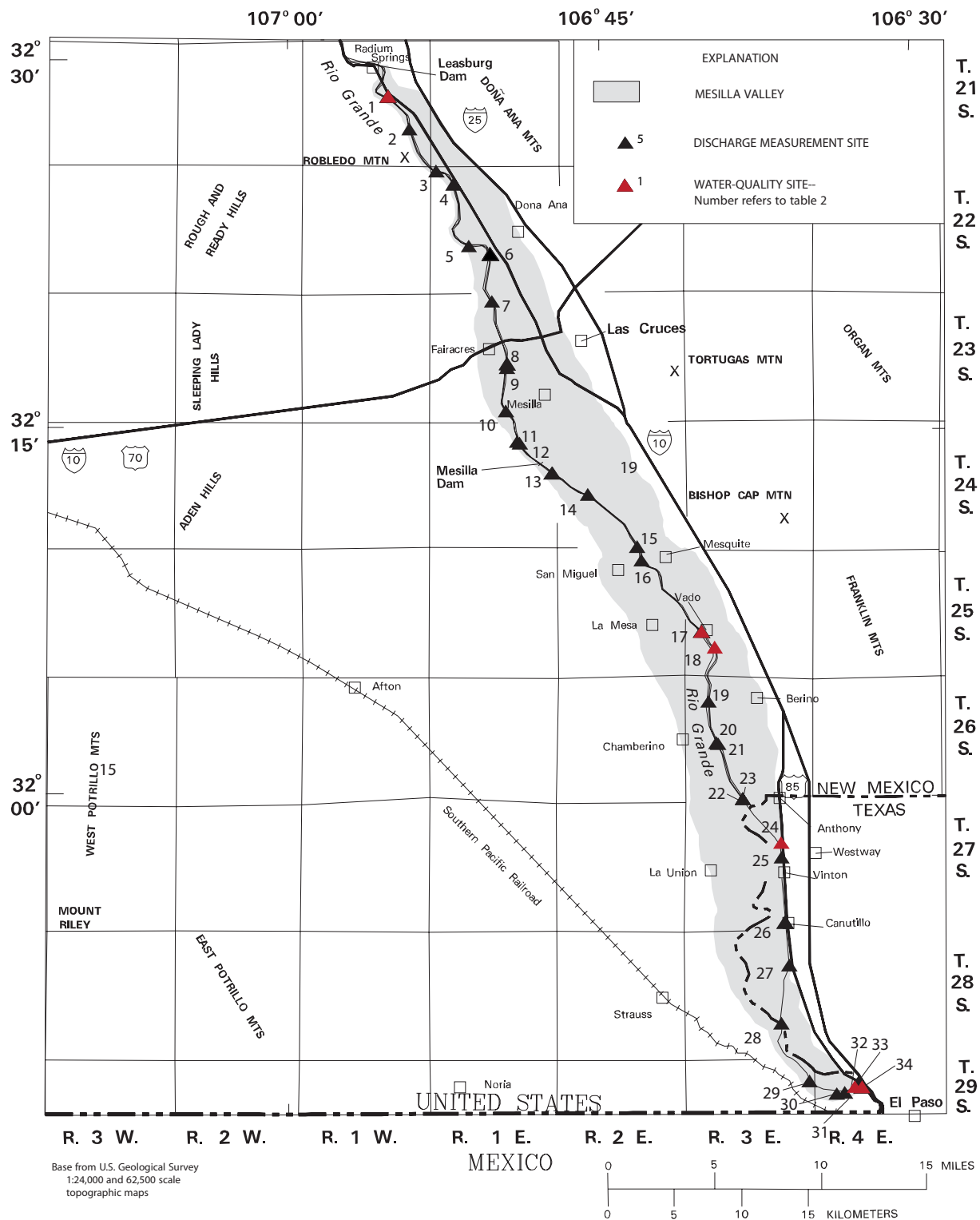
Figure 2.--Location of discharge measurement sites and water-quality sites during seepage investigations of the Rio Grande from Radium Springs, New Mexico, to El Paso, Texas, water years 2004 through 2006 (modified from Nickerson, 1995, fig. 8).
