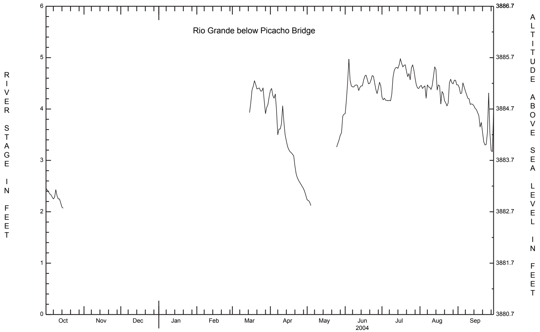
Mean daily river stage of the Rio Grande below Picacho Bridge, 2004 water year.
