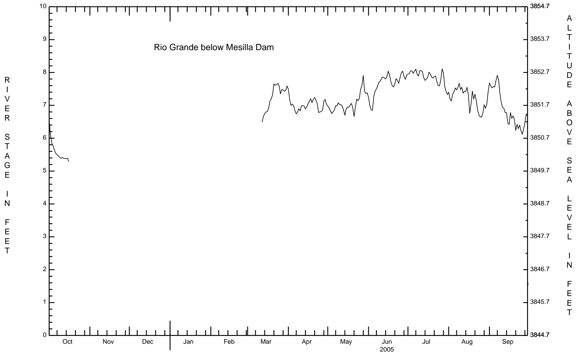
Mean daily river stage of the Rio Grande below Mesilla Dam, 2005 water year.
