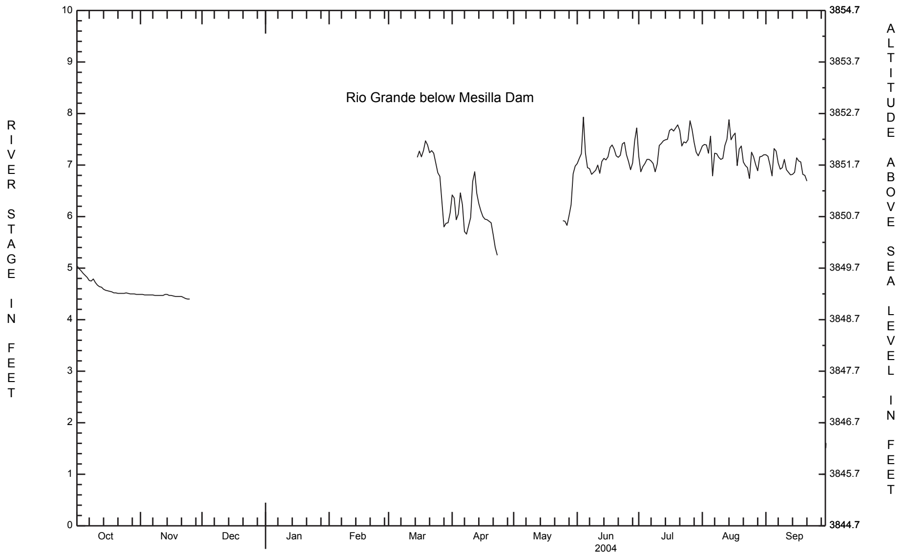
Mean daily river stage of the Rio Grande below Mesilla Dam, 2004 water year.
