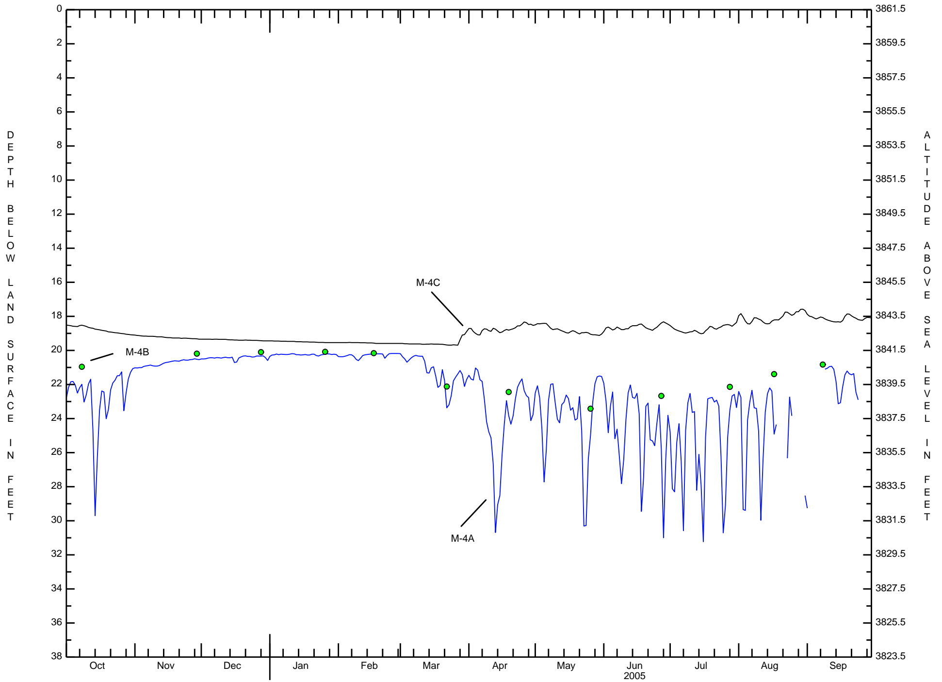
Mean daily water levels and miscellaneous water levels in well group M-4, 2005 water year.
