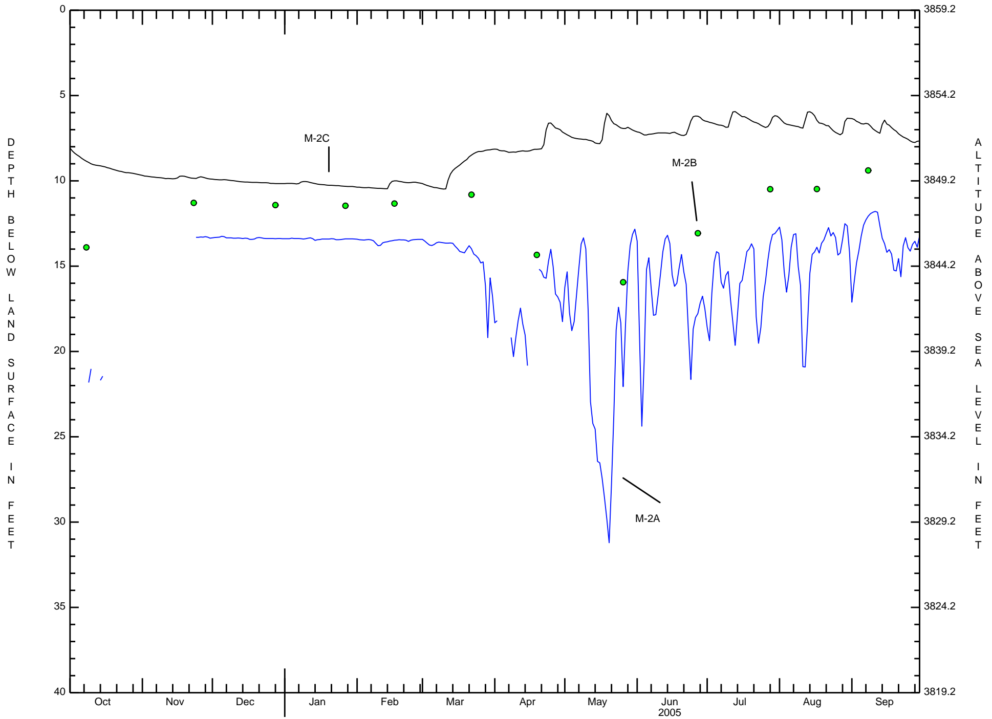
Mean daily water levels and miscellaneous water levels in well group M-2, 2005 water year.
