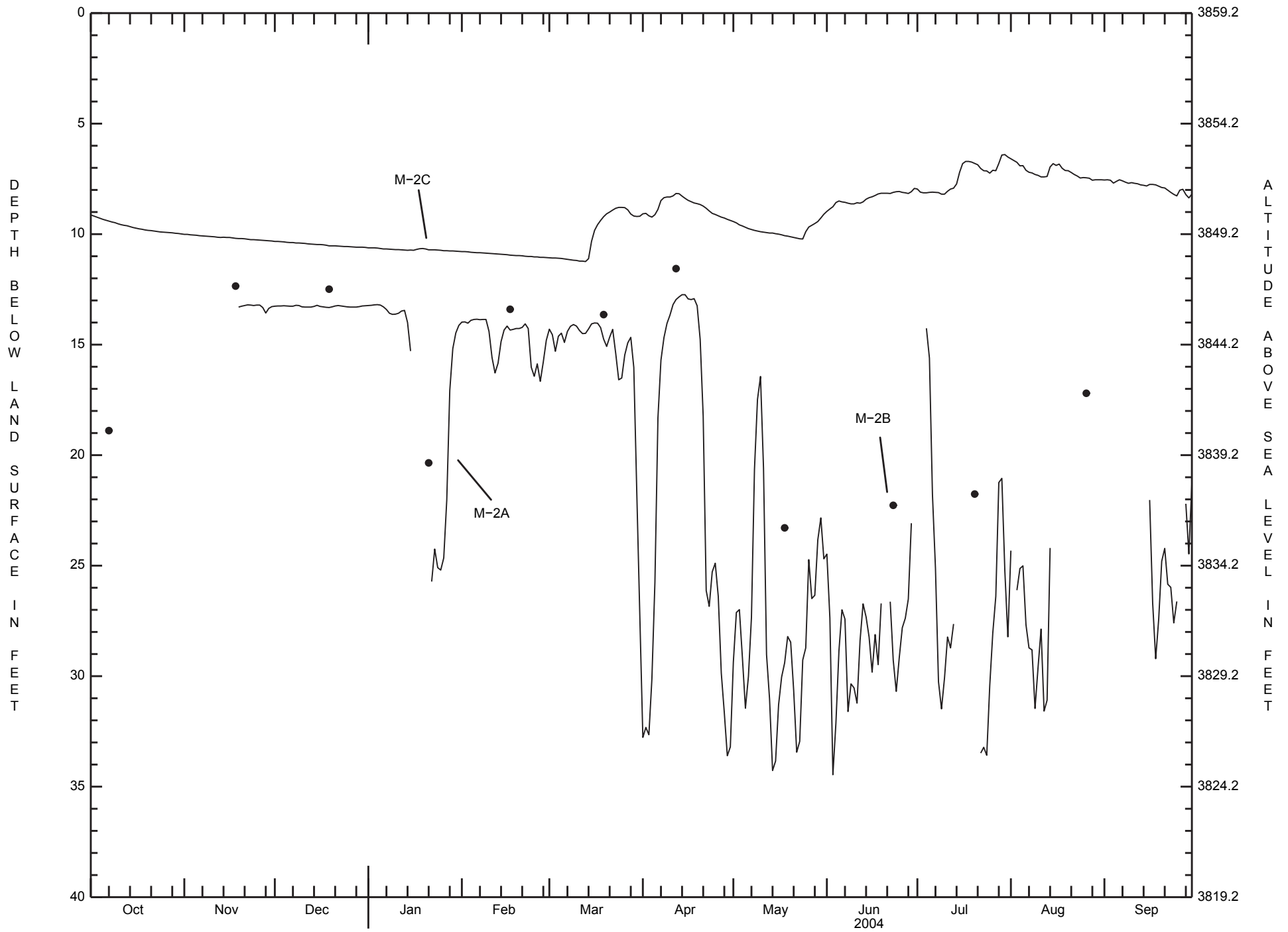
Mean daily water levels and miscellaneous water levels in well group M-2, 2004 water year.
